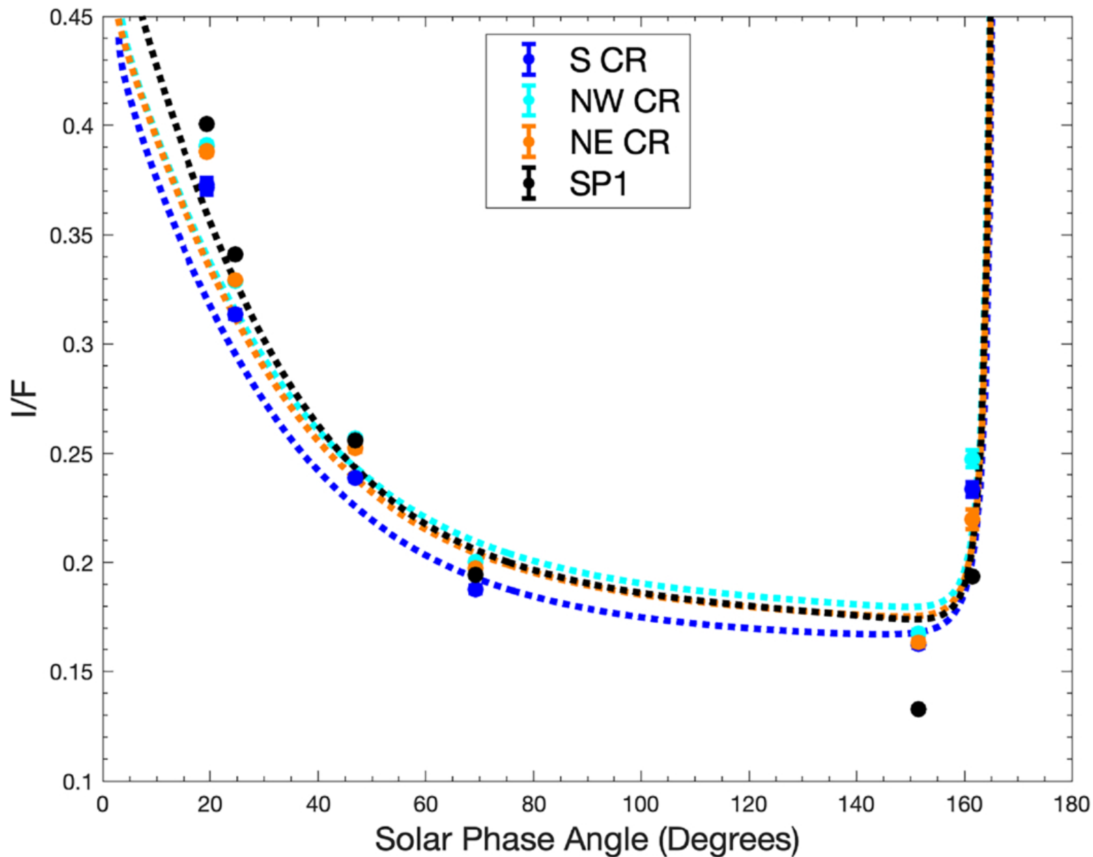
Figure 7. from Jason D. Hofgartner et al 2025 Planet. Sci. J. 6 doi:10.3847/PSJ/ade87c https://dx.doi.org/10.3847/PSJ/ade87c © 2025. The Author(s). Published by the American Astronomical Society.
