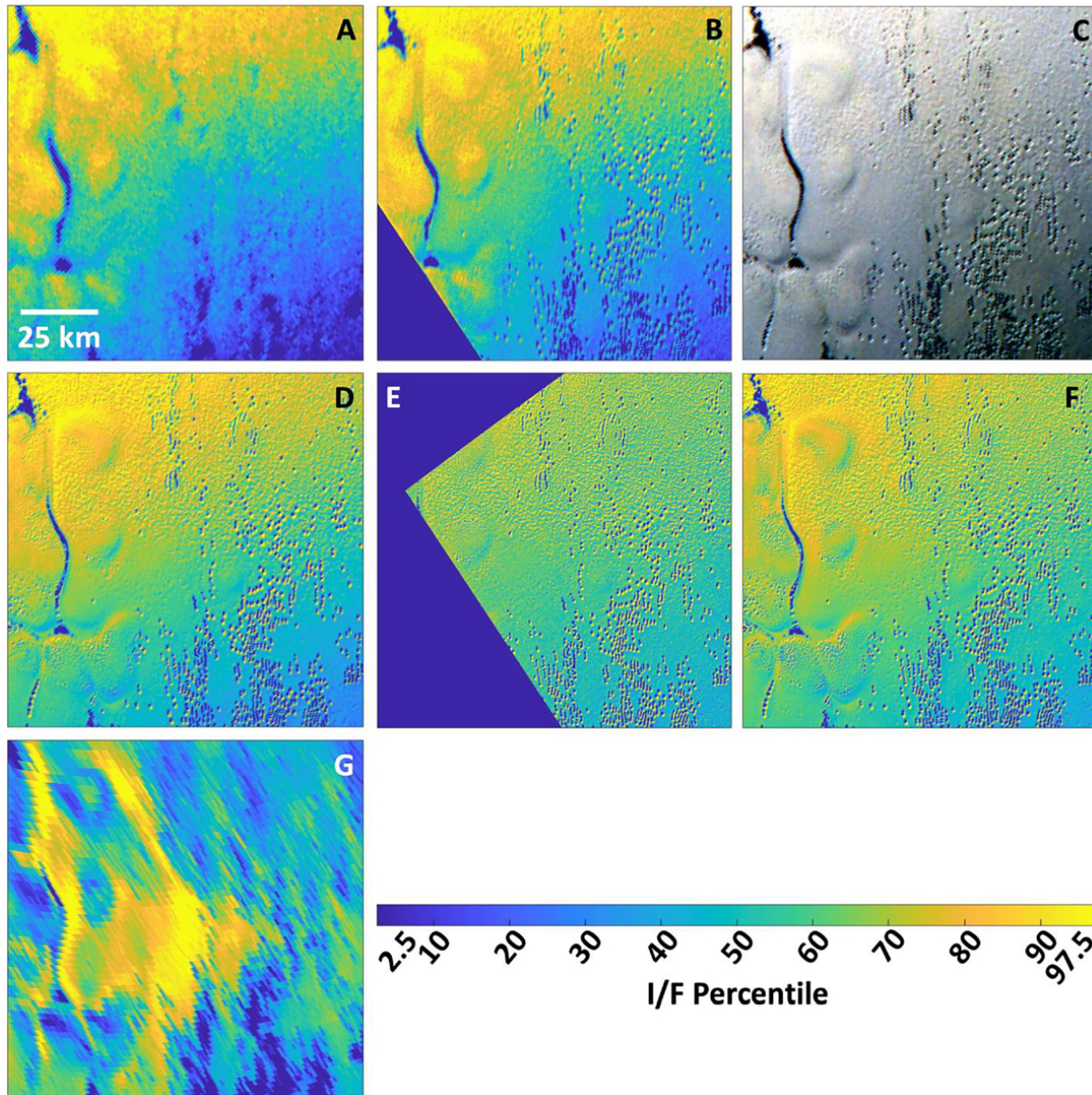
Figure 6. from Jason D. Hofgartner et al 2025 Planet. Sci. J. 6 doi:10.3847/PSJ/ade87c https://dx.doi.org/10.3847/PSJ/ade87c © 2025. The Author(s). Published by the American Astronomical Society.
