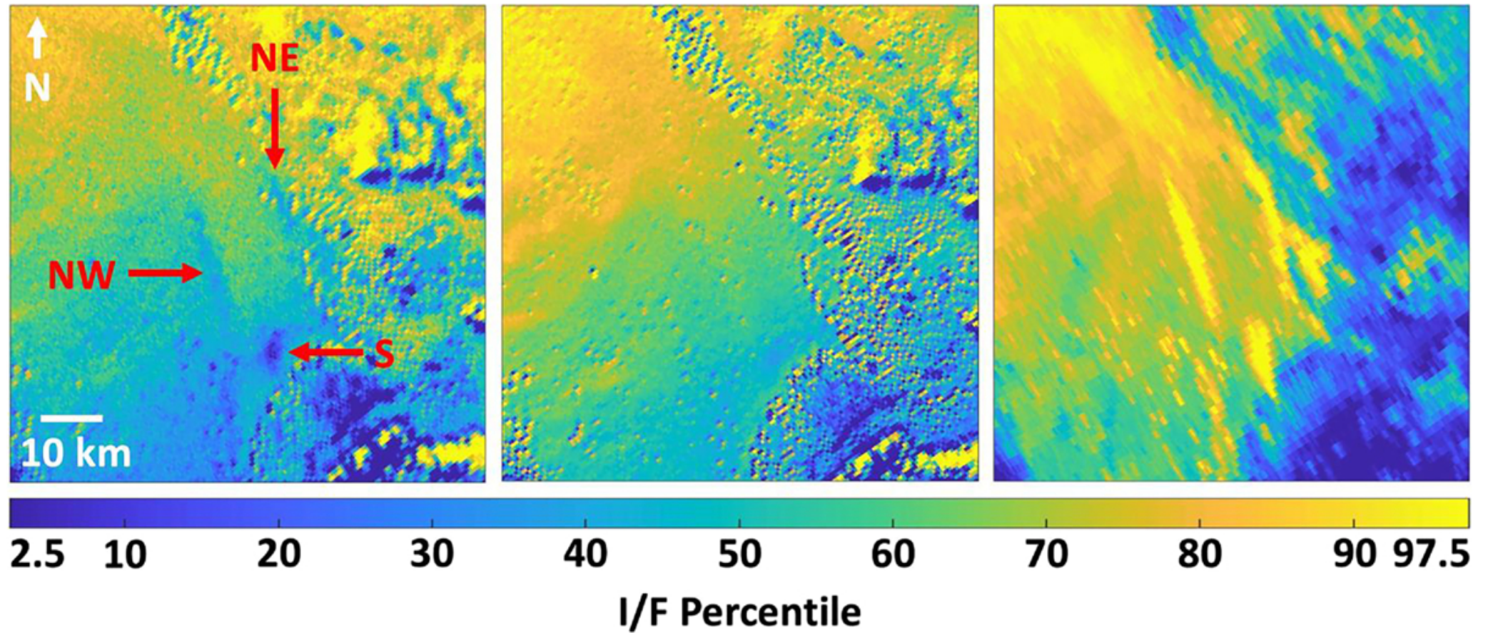
Figure 1. from Jason D. Hofgartner et al 2025 Planet. Sci. J. 6 doi:10.3847/PSJ/ade87c https://dx.doi.org/10.3847/PSJ/ade87c © 2025. The Author(s). Published by the American Astronomical Society.
