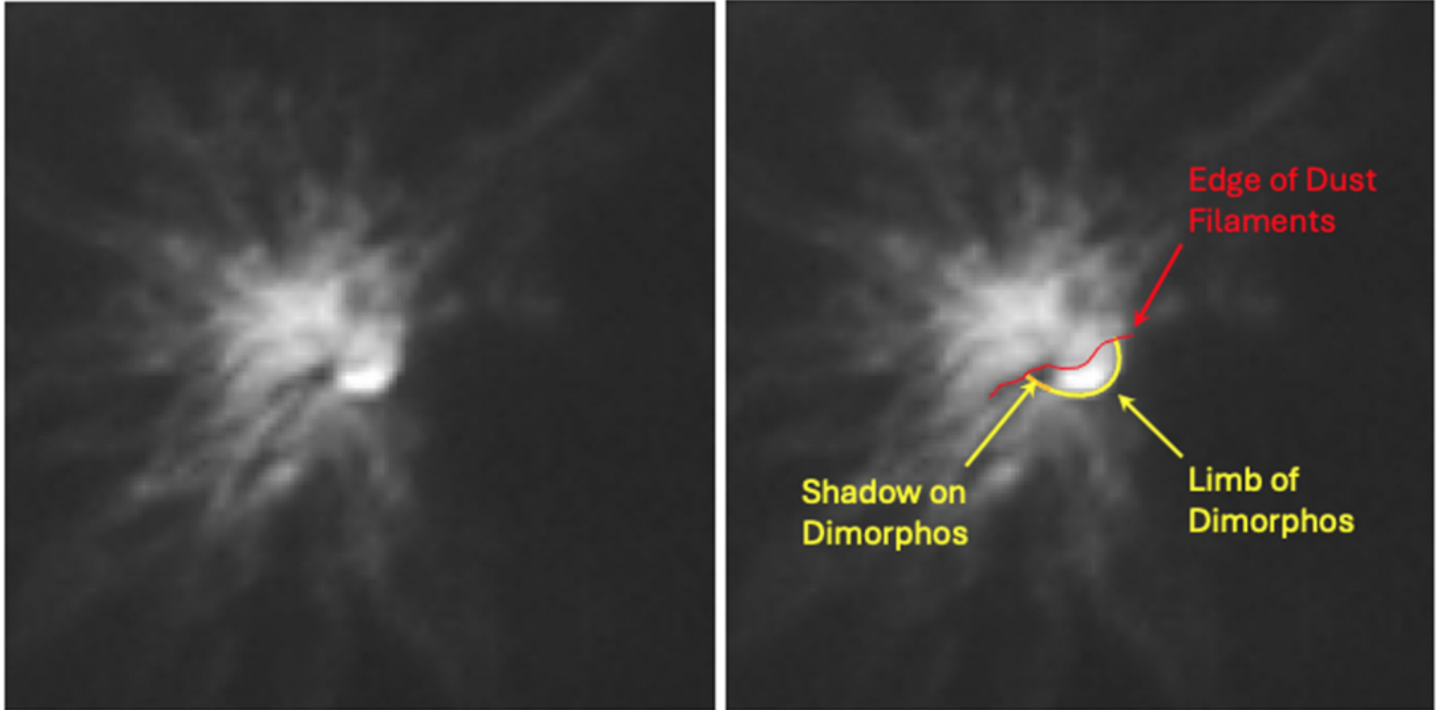
Figure 5. from Tony L. Farnham et al 2025 Planet. Sci. J. 6 doi:10.3847/PSJ/addd1a https://dx.doi.org/10.3847/PSJ/addd1a © 2025. The Author(s). Published by the American Astronomical Society.
