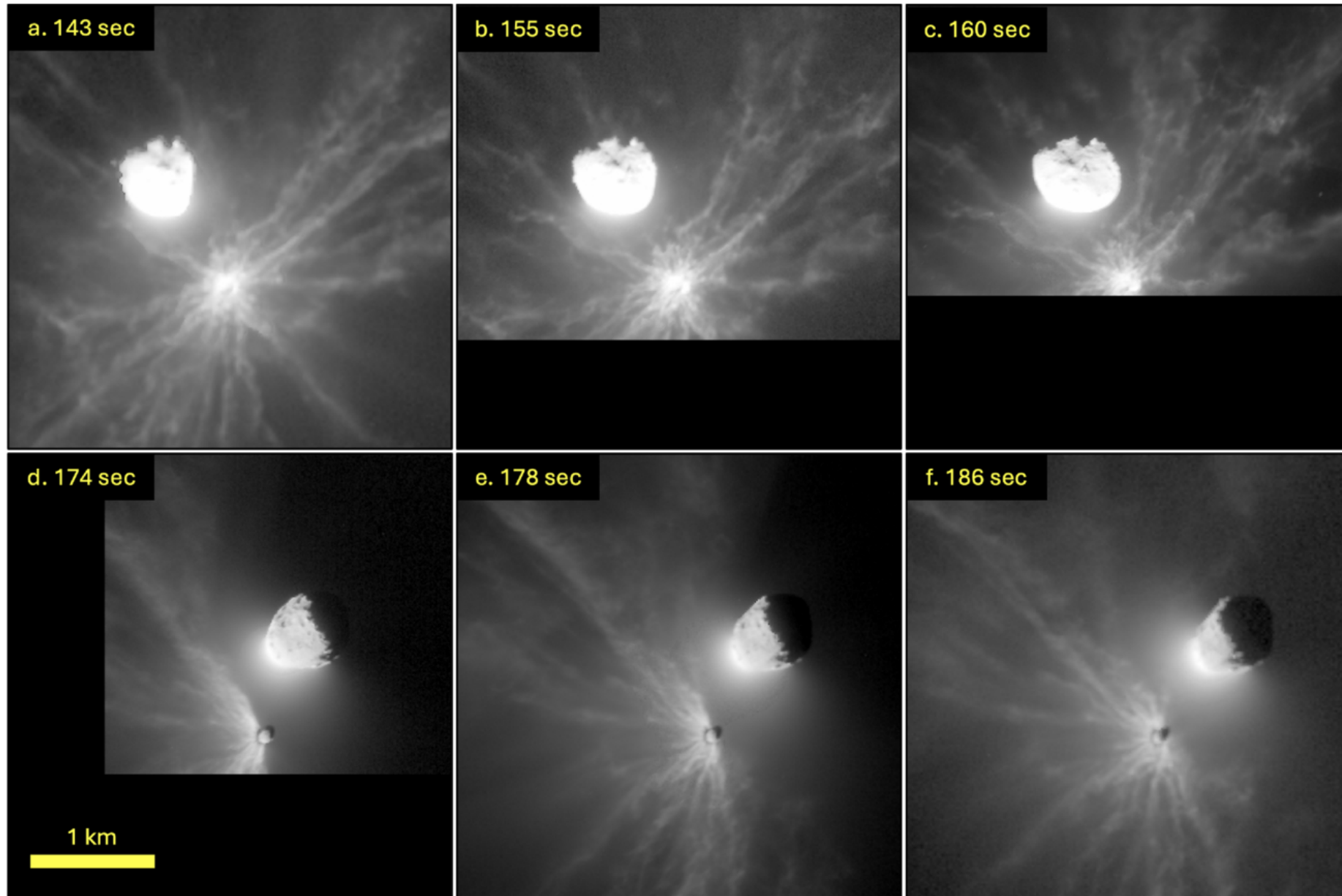
Figure 4. from Tony L. Farnham et al 2025 Planet. Sci. J. 6 doi:10.3847/PSJ/addd1a https://dx.doi.org/10.3847/PSJ/addd1a © 2025. The Author(s). Published by the American Astronomical Society.
