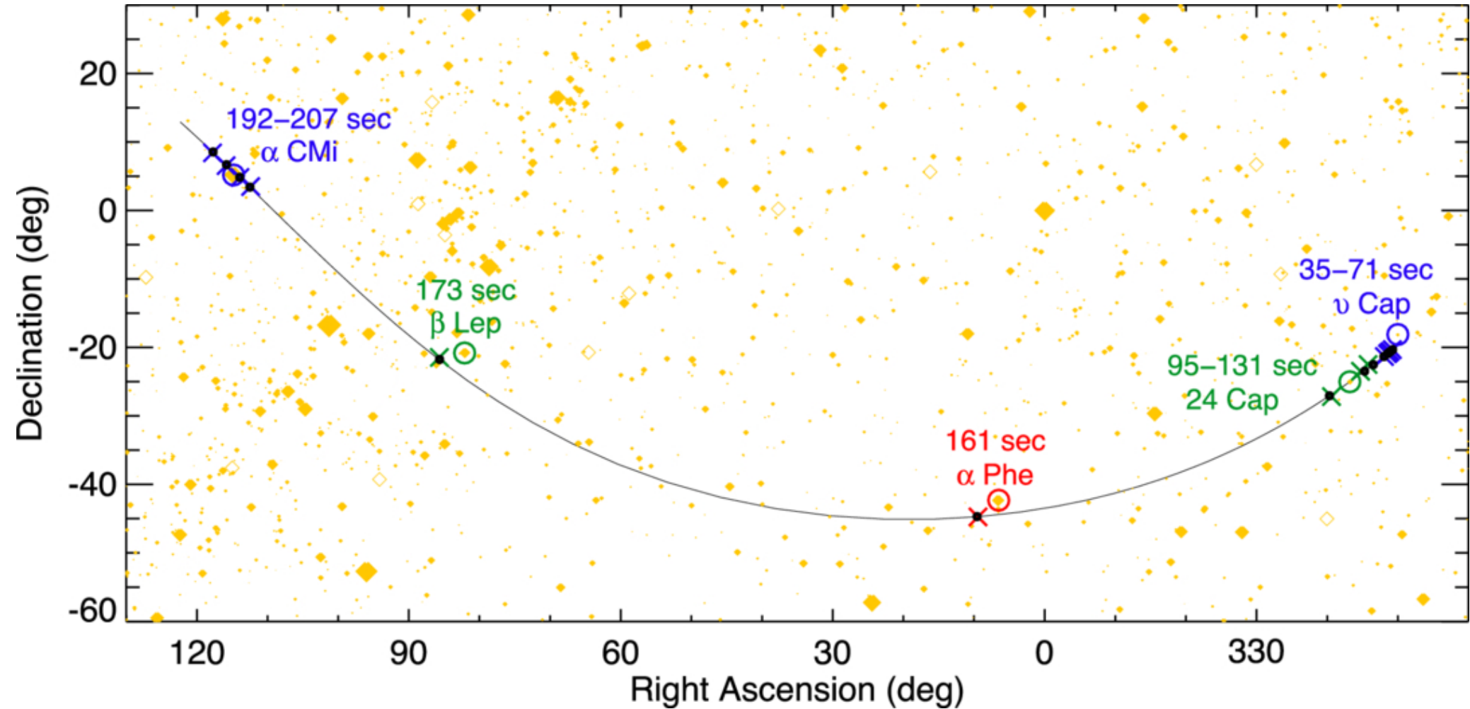
Figure 14. from Tony L. Farnham et al 2025 Planet. Sci. J. 6 doi:10.3847/PSJ/addd1a https://dx.doi.org/10.3847/PSJ/addd1a © 2025. The Author(s). Published by the American Astronomical Society.
