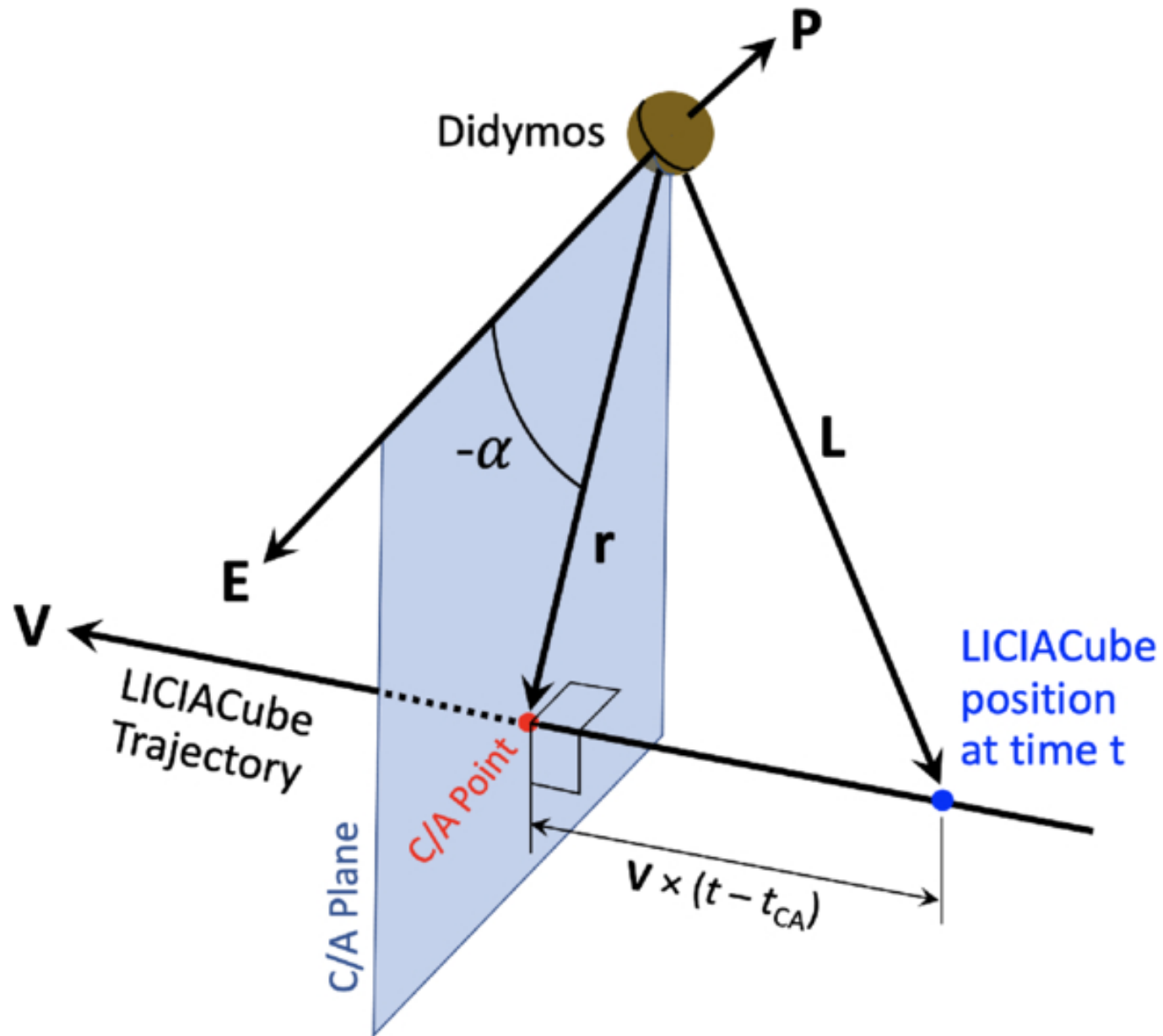
Figure 13. from Tony L. Farnham et al 2025 Planet. Sci. J. 6 doi:10.3847/PSJ/addd1a https://dx.doi.org/10.3847/PSJ/addd1a © 2025. The Author(s). Published by the American Astronomical Society.
