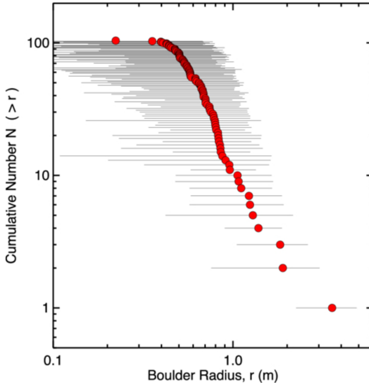
Figure 10. from Tony L. Farnham et al 2025 Planet. Sci. J. 6 doi:10.3847/PSJ/addd1a https://dx.doi.org/10.3847/PSJ/addd1a © 2025. The Author(s). Published by the American Astronomical Society.
