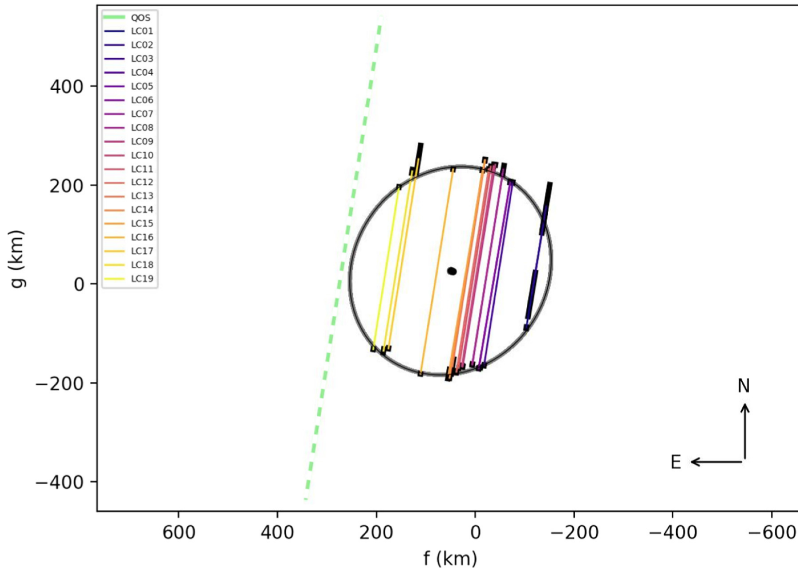
Figure 9. from F. L. Rommel et al 2025 Planet. Sci. J. 6 doi:10.3847/PSJ/adabc1 https://dx.doi.org/10.3847/PSJ/adabc1 © 2025. The Author(s). Published by the American Astronomical Society.
