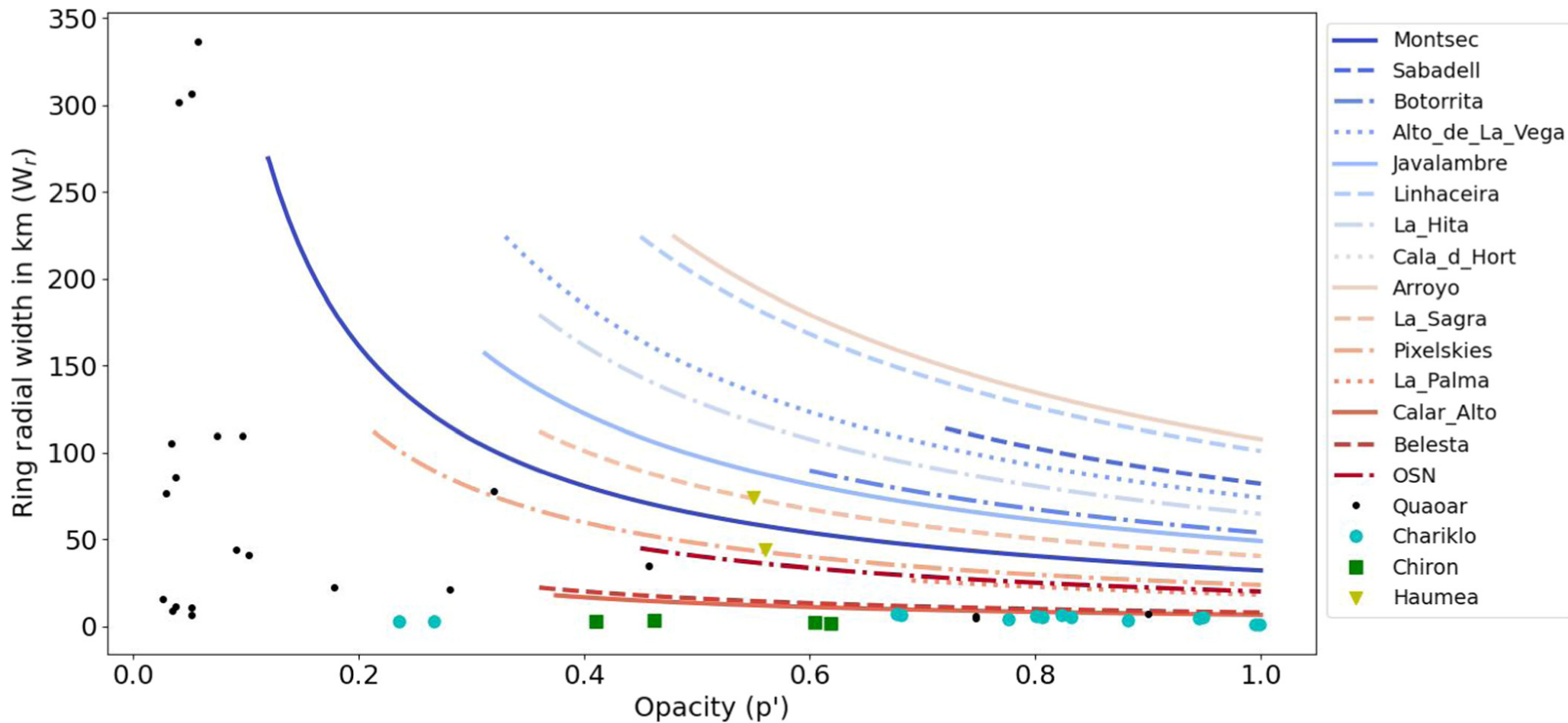
Figure 7. from F. L. Rommel et al 2025 Planet. Sci. J. 6 doi:10.3847/PSJ/adabc1 https://dx.doi.org/10.3847/PSJ/adabc1 © 2025. The Author(s). Published by the American Astronomical Society.
