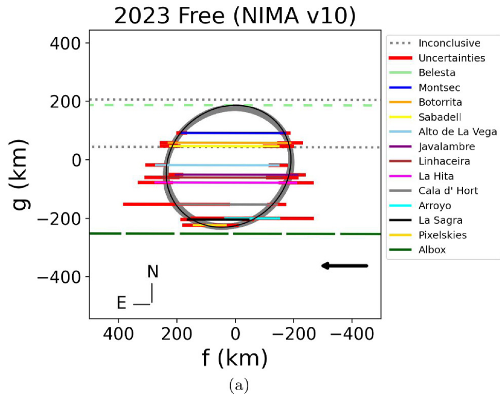
Figure 4. from F. L. Rommel et al 2025 Planet. Sci. J. 6 doi:10.3847/PSJ/adabc1 https://dx.doi.org/10.3847/PSJ/adabc1 © 2025. The Author(s). Published by the American Astronomical Society.
