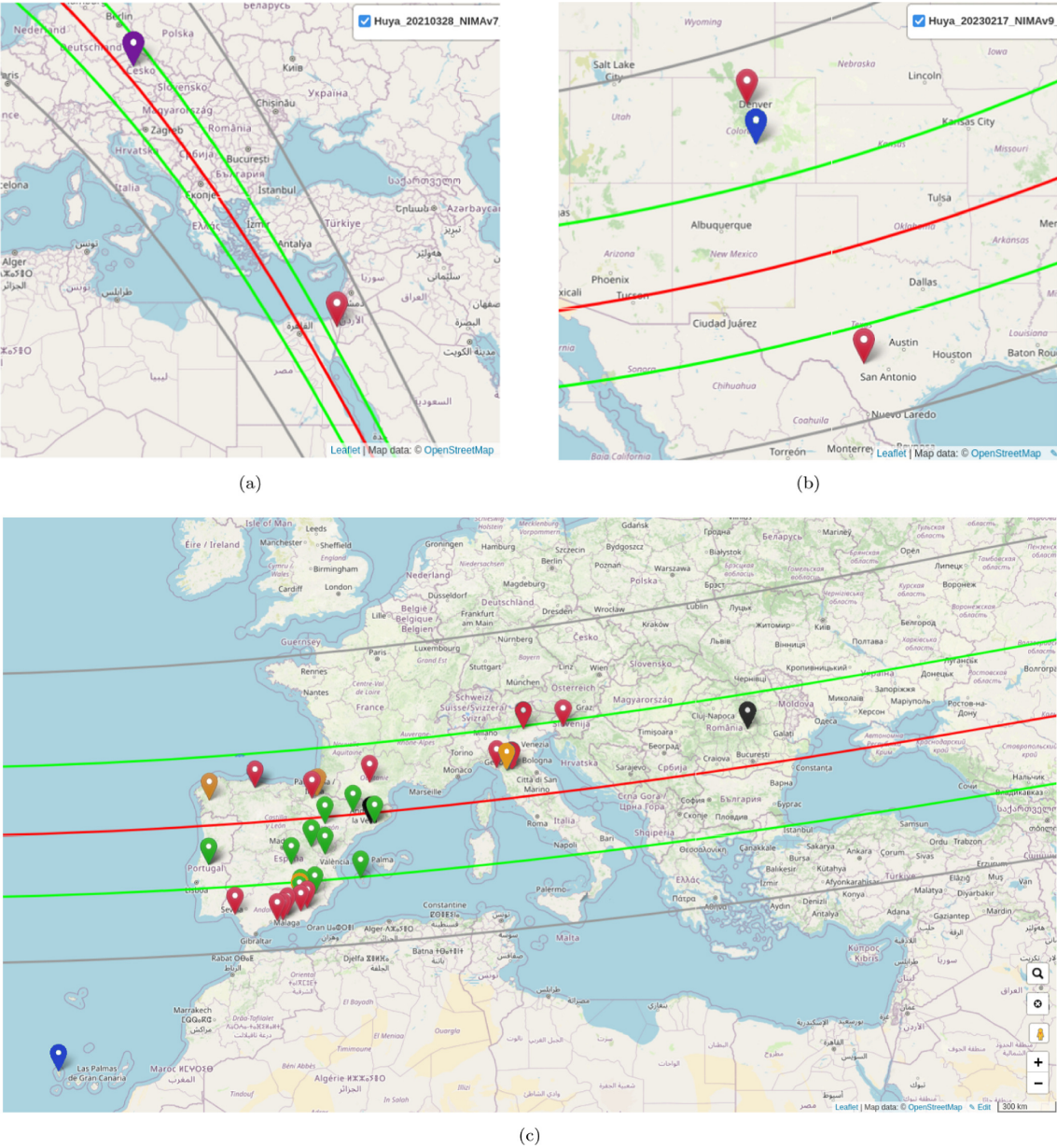
Figure 2. from F. L. Rommel et al 2025 Planet. Sci. J. 6 doi:10.3847/PSJ/adabc1 https://dx.doi.org/10.3847/PSJ/adabc1 © 2025. The Author(s). Published by the American Astronomical Society.
