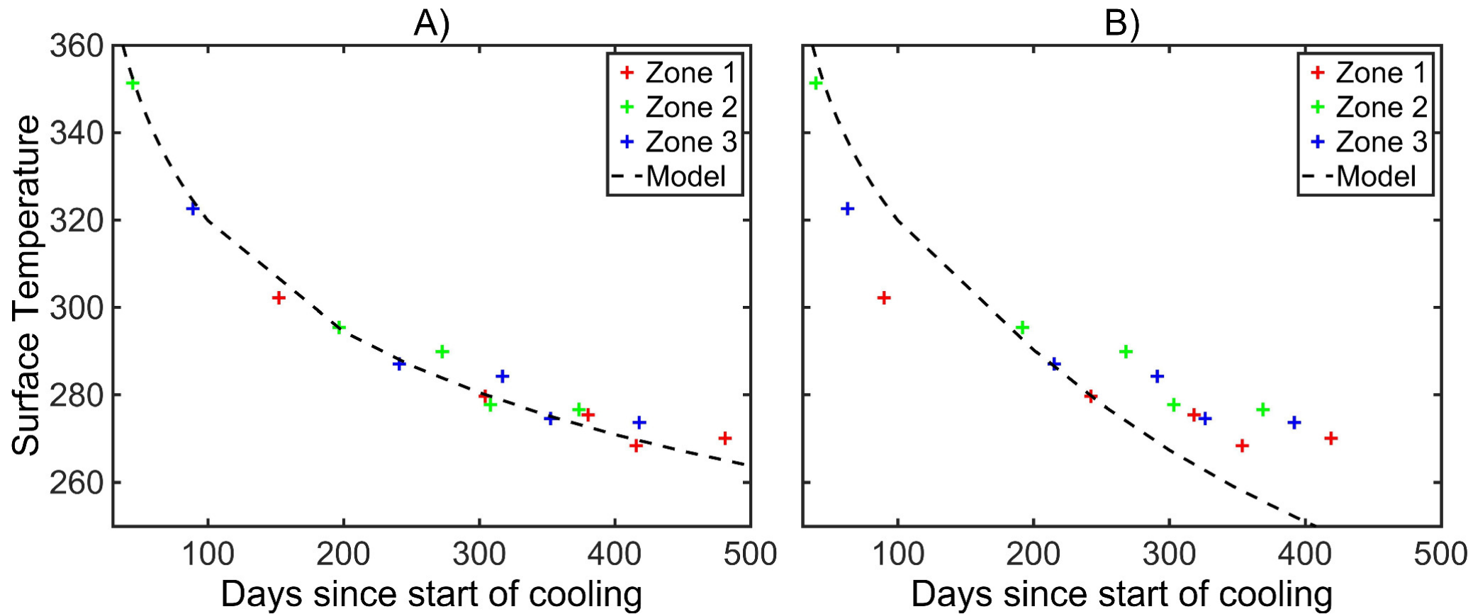
Figure A3. from Alessandro Mura et al 2025 Planet. Sci. J. 6 doi:10.3847/PSJ/ada27c https://dx.doi.org/10.3847/PSJ/ada27c © 2025. The Author(s). Published by the American Astronomical Society.
