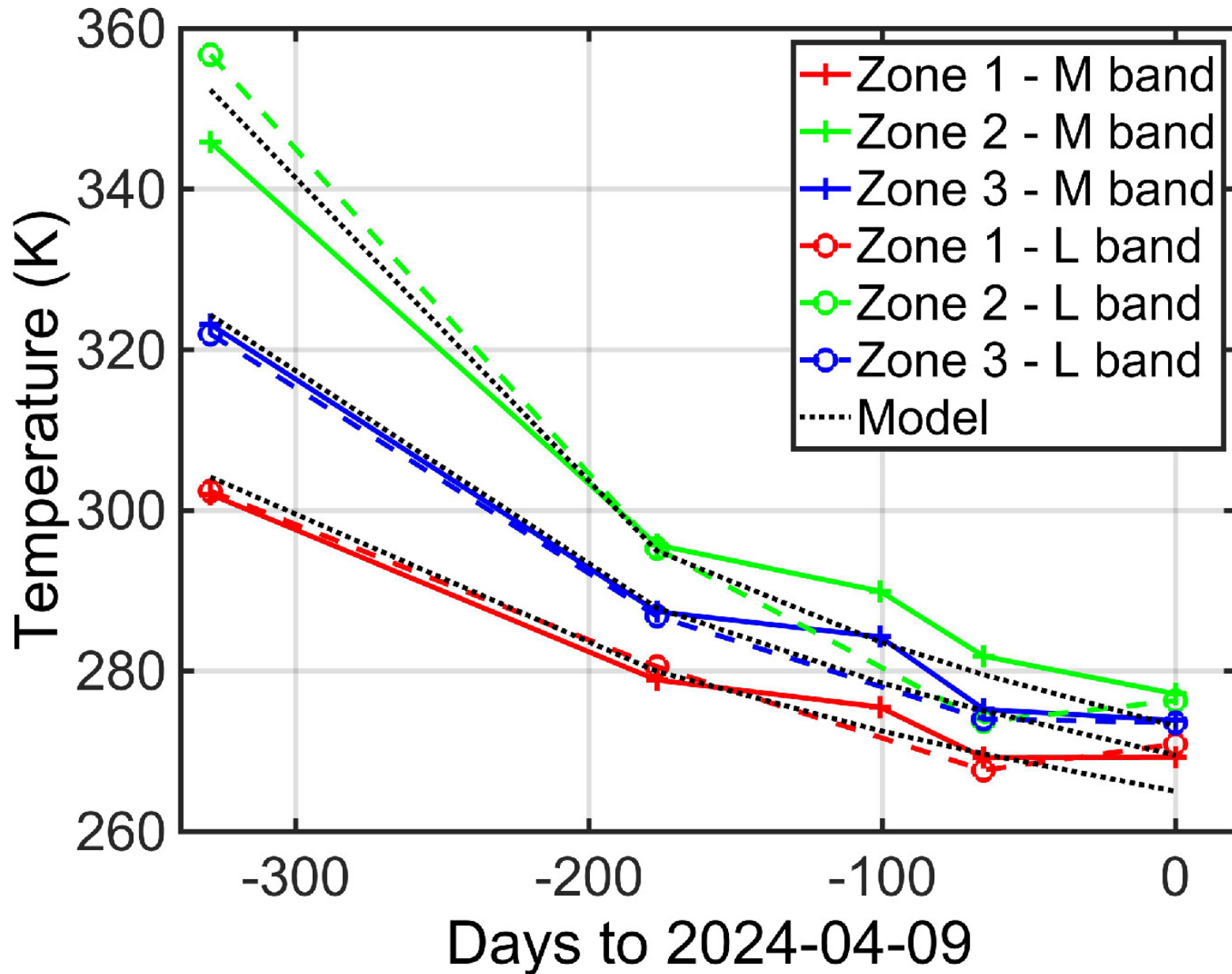
Figure 2. from Alessandro Mura et al 2025 Planet. Sci. J. 6 doi:10.3847/PSJ/ada27c https://dx.doi.org/10.3847/PSJ/ada27c © 2025. The Author(s). Published by the American Astronomical Society.
