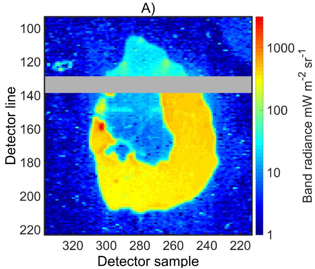
Figure A6. from Alessandro Mura et al 2025 Planet. Sci. J. 6 doi:10.3847/PSJ/ada27c https://dx.doi.org/10.3847/PSJ/ada27c © 2025. The Author(s). Published by the American Astronomical Society.
