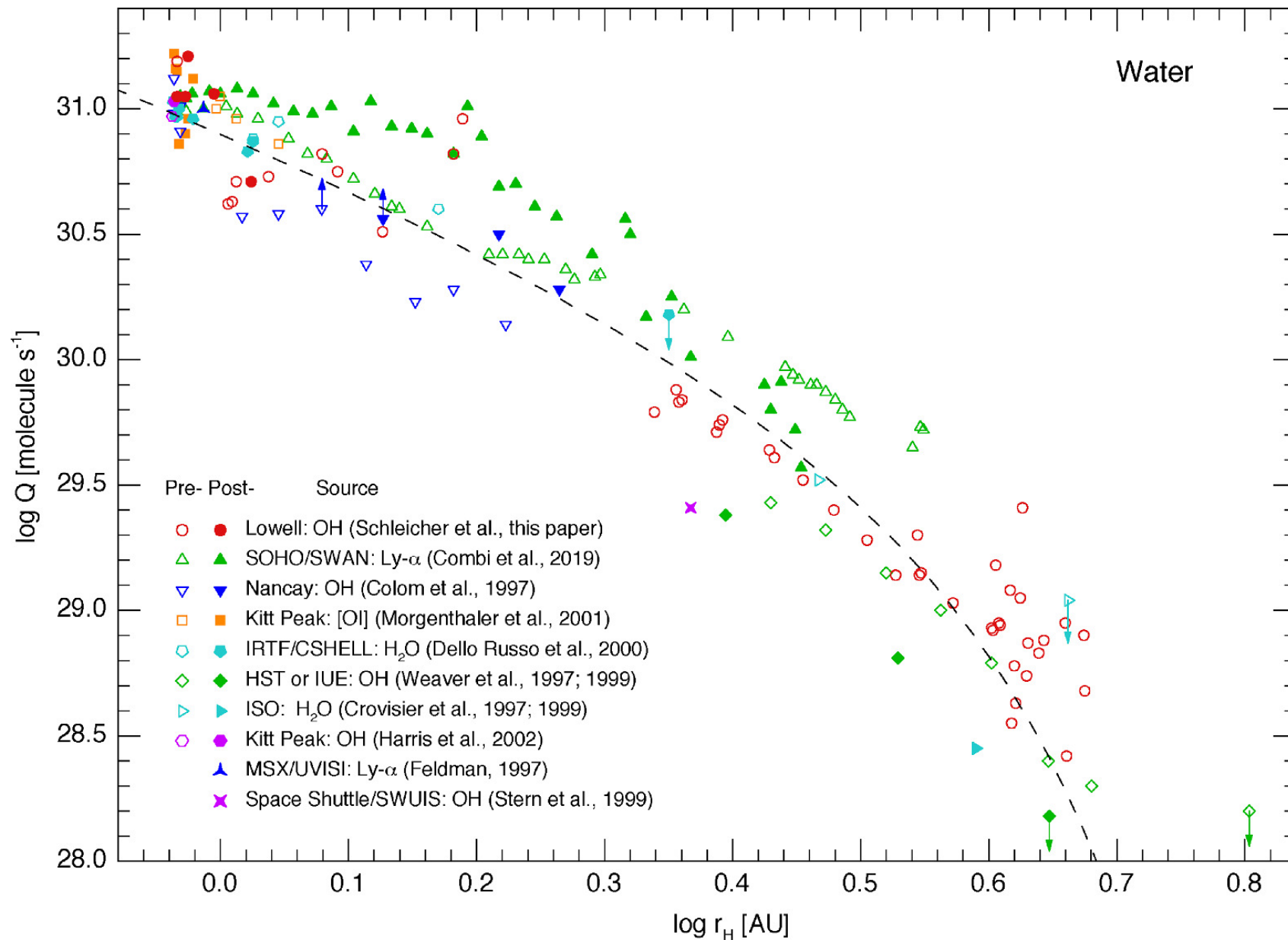
Figure 6. from David G. Schleicher et al 2024 Planet. Sci. J. 5 doi:10.3847/PSJ/ad86b9 https://dx.doi.org/10.3847/PSJ/ad86b9 © 2024. The Author(s). Published by the American Astronomical Society.
