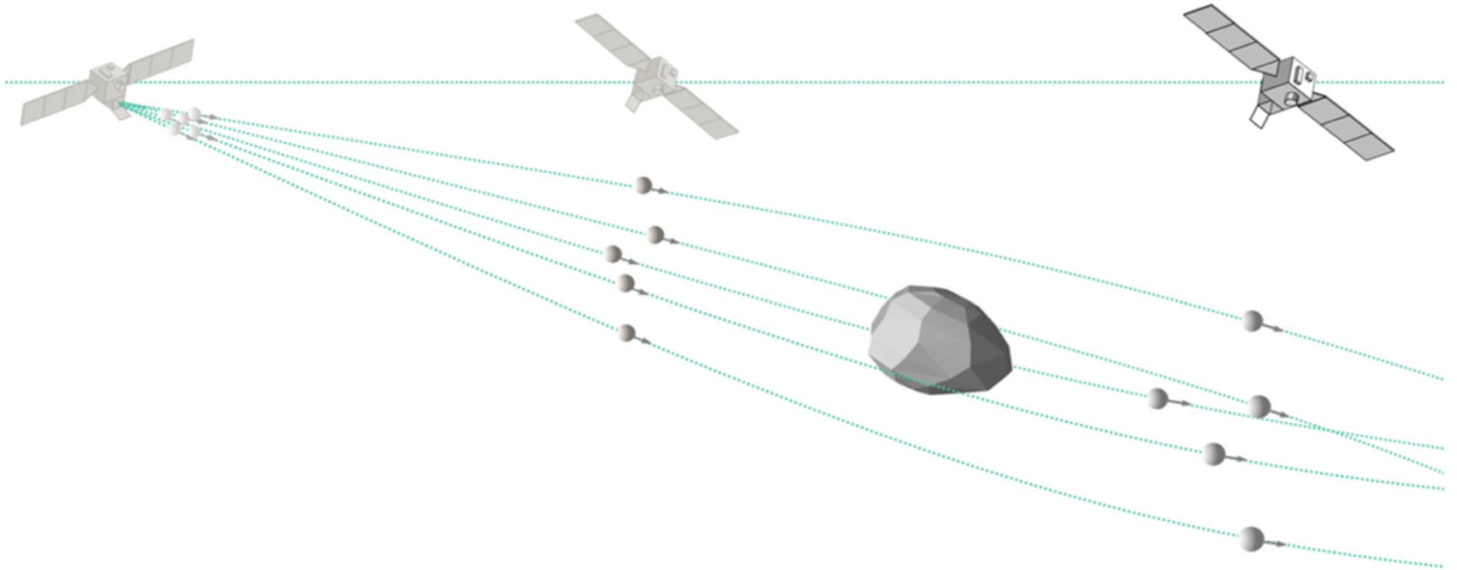
Figure 2. from Angela M. Stickle et al 2024 Planet. Sci. J. 5 doi:10.3847/PSJ/ad7a6c https://dx.doi.org/10.3847/PSJ/ad7a6c © 2024. The Author(s). Published by the American Astronomical Society.
