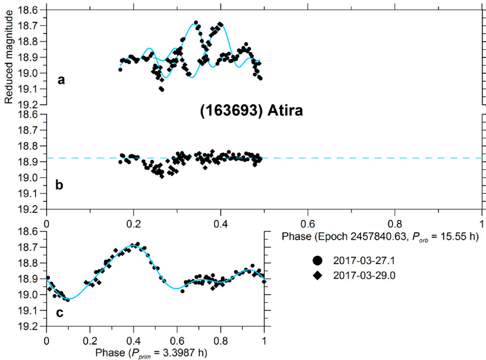
Figure 9. from Aaron P. Deleon et al 2024 Planet. Sci. J. 5 doi:10.3847/PSJ/ad7814 https://dx.doi.org/10.3847/PSJ/ad7814 © 2024. The Author(s). Published by the American Astronomical Society.
