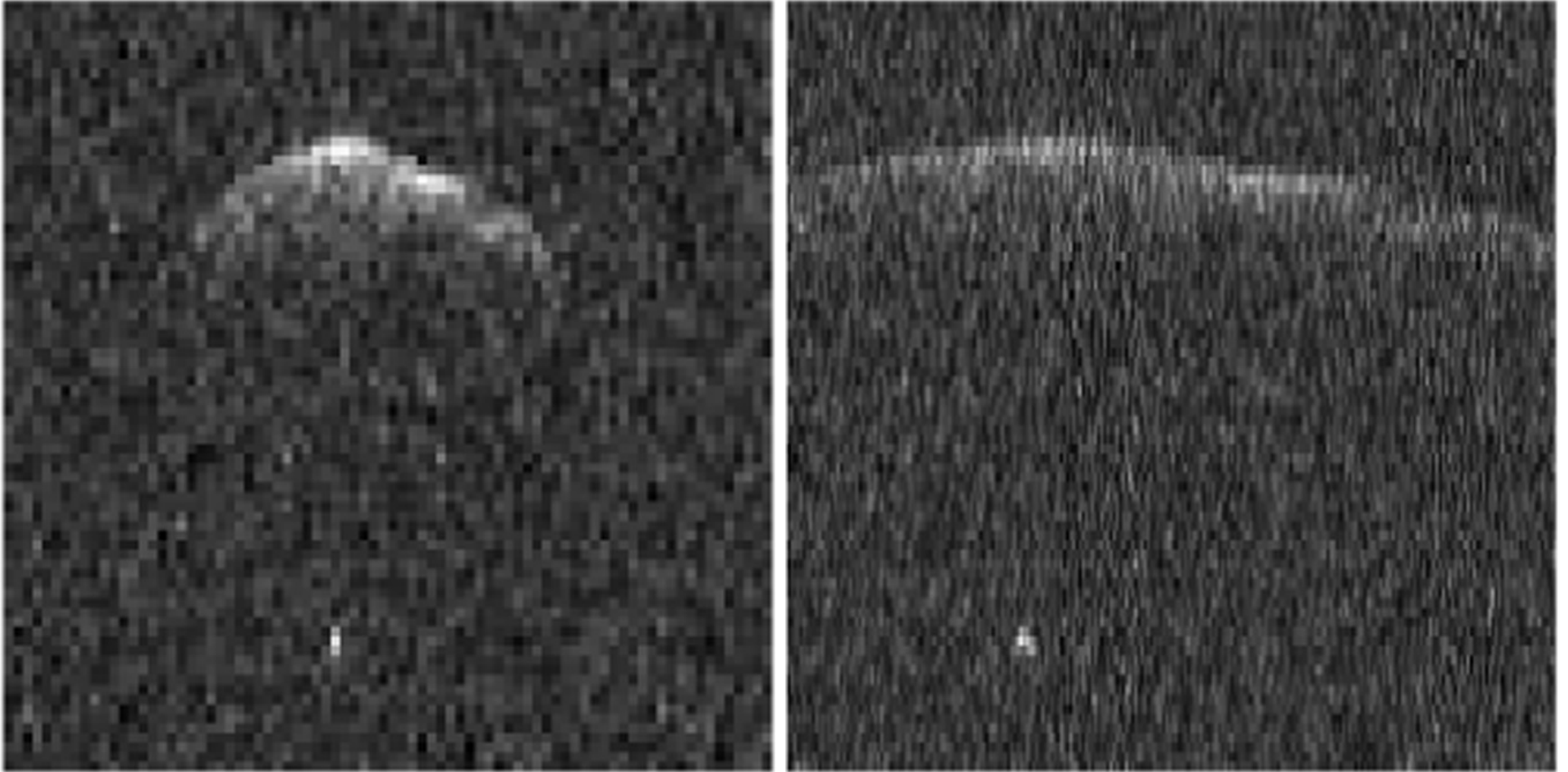
Figure 3. from Aaron P. Deleon et al 2024 Planet. Sci. J. 5 doi:10.3847/PSJ/ad7814 https://dx.doi.org/10.3847/PSJ/ad7814 © 2024. The Author(s). Published by the American Astronomical Society.
