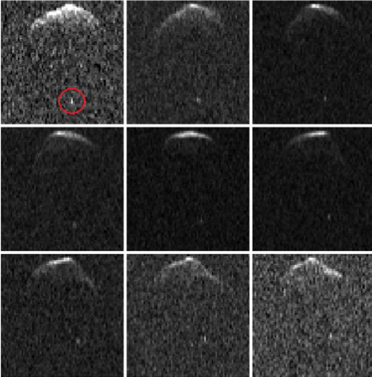
Figure 2. from Aaron P. Deleon et al 2024 Planet. Sci. J. 5 doi:10.3847/PSJ/ad7814 https://dx.doi.org/10.3847/PSJ/ad7814 © 2024. The Author(s). Published by the American Astronomical Society.
