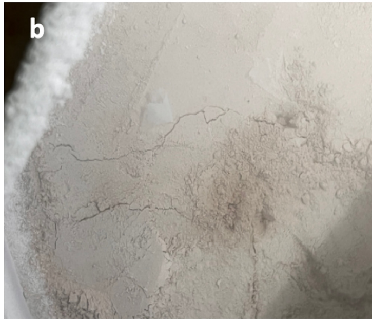
Figure 9. from Lauren E. Mc Keown et al 2024 Planet. Sci. J. 5 doi:10.3847/PSJ/ad67c8 https://dx.doi.org/10.3847/PSJ/ad67c8 © 2024. The Author(s). Published by the American Astronomical Society.
