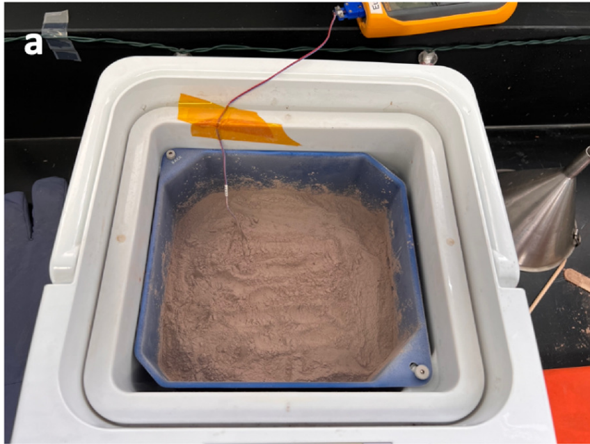
Figure 3. from Lauren E. Mc Keown et al 2024 Planet. Sci. J. 5 doi:10.3847/PSJ/ad67c8 https://dx.doi.org/10.3847/PSJ/ad67c8 © 2024. The Author(s). Published by the American Astronomical Society.
