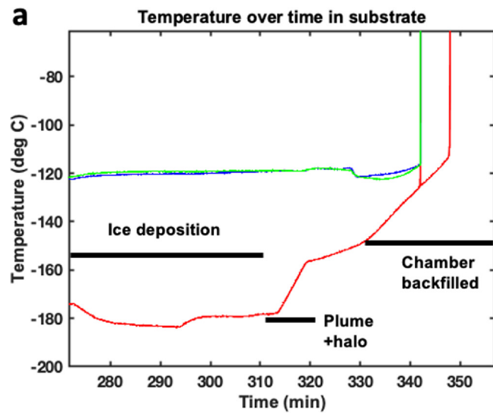
Figure 11. from Lauren E. Mc Keown et al 2024 Planet. Sci. J. 5 doi:10.3847/PSJ/ad67c8 https://dx.doi.org/10.3847/PSJ/ad67c8 © 2024. The Author(s). Published by the American Astronomical Society.
