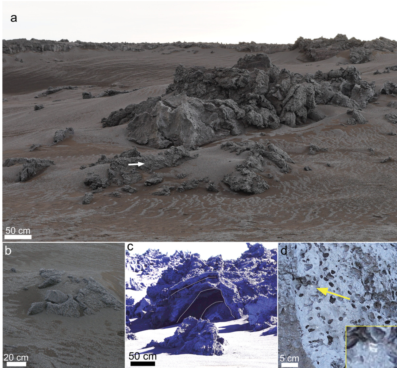
Figure 9. from Samantha Gwizd et al 2024 Planet. Sci. J. 5 doi:10.3847/PSJ/ad55f4 https://dx.doi.org/10.3847/PSJ/ad55f4 © 2024. The Author(s). Published by the American Astronomical Society.
