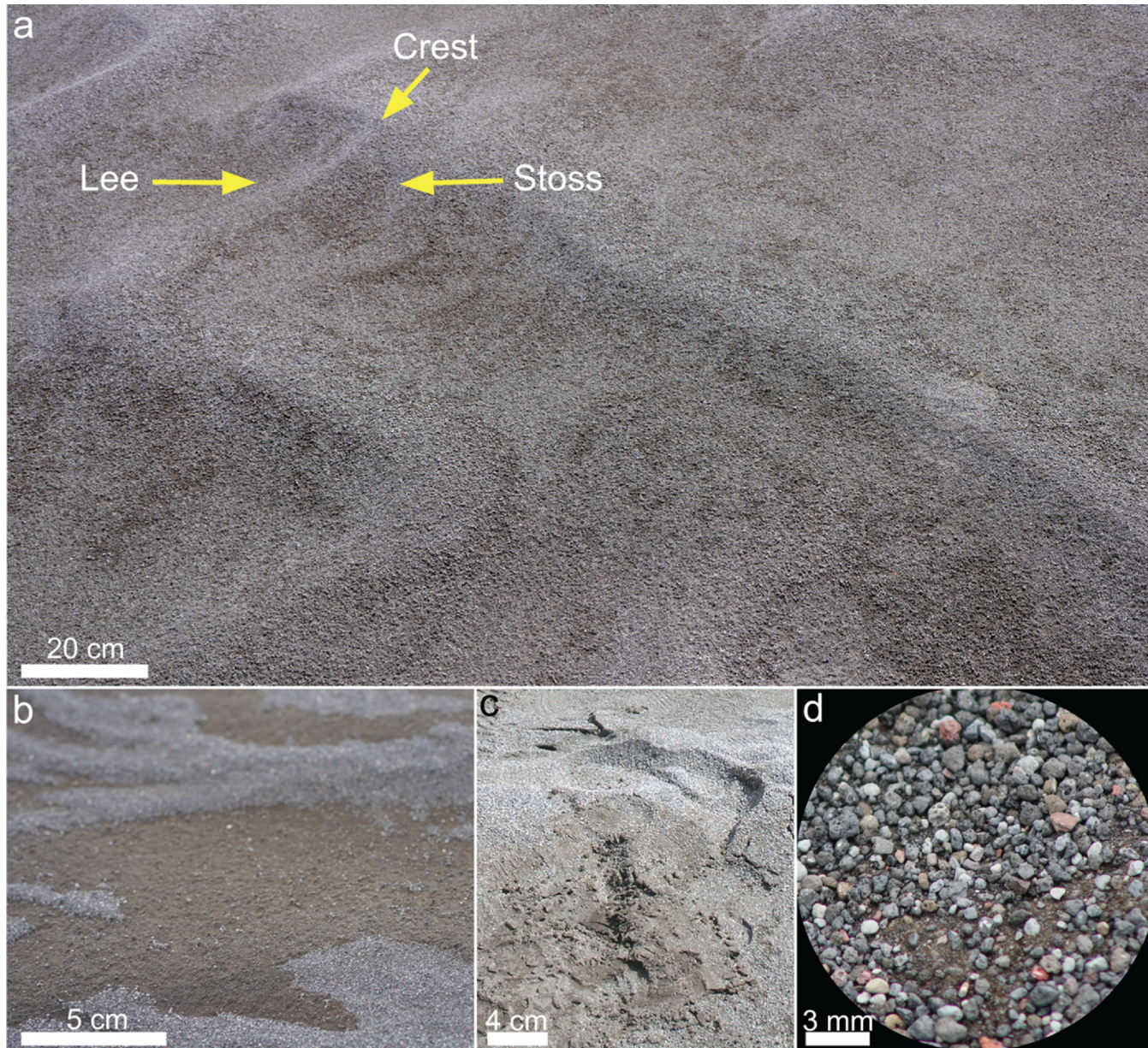
Figure 8. from Samantha Gwizd et al 2024 Planet. Sci. J. 5 doi:10.3847/PSJ/ad55f4 https://dx.doi.org/10.3847/PSJ/ad55f4 © 2024. The Author(s). Published by the American Astronomical Society.
