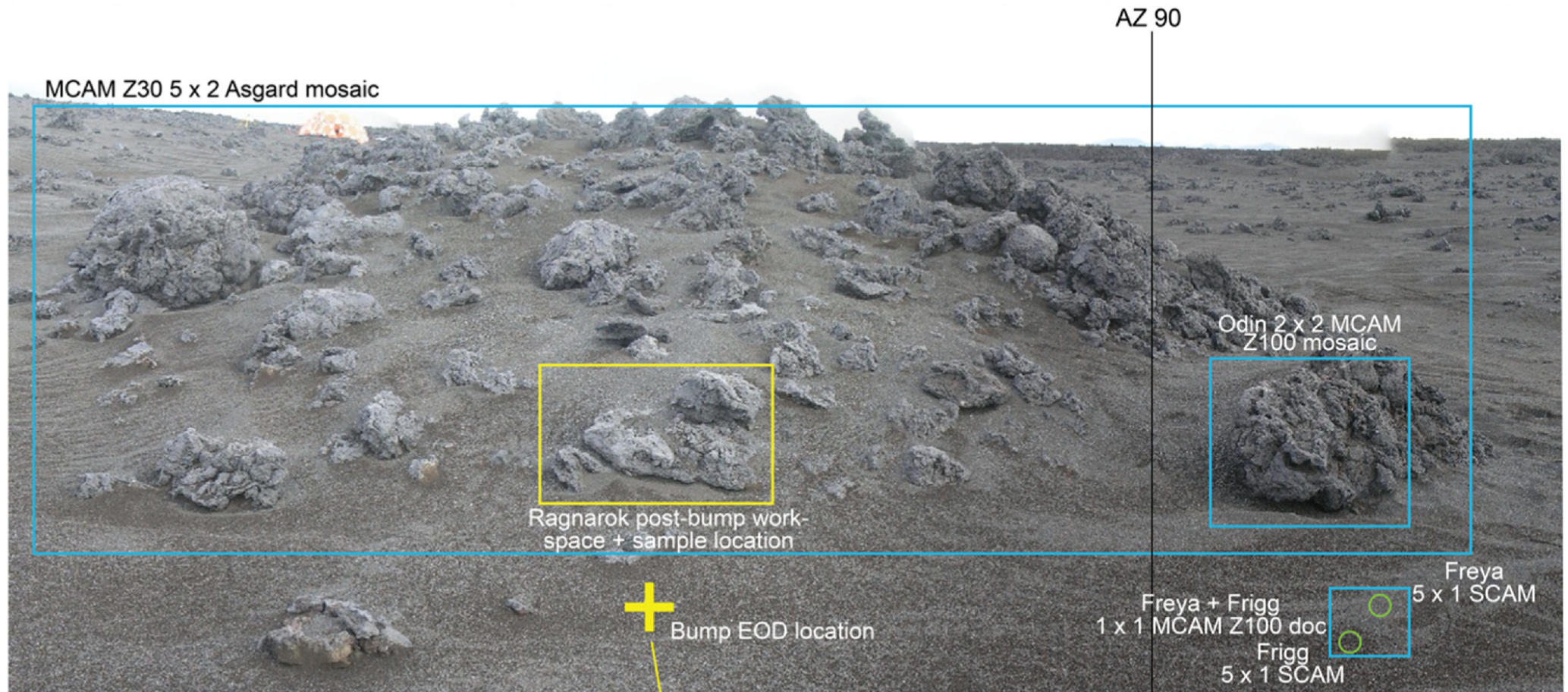
Figure 5. from Samantha Gwizd et al 2024 Planet. Sci. J. 5 doi:10.3847/PSJ/ad55f4 https://dx.doi.org/10.3847/PSJ/ad55f4 © 2024. The Author(s). Published by the American Astronomical Society.
