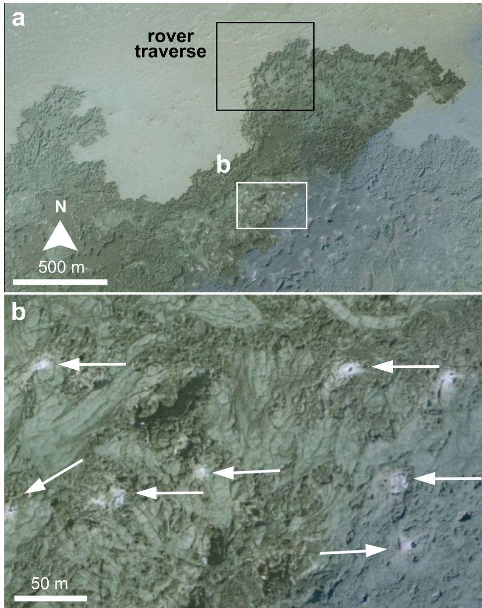
Figure A1. from Samantha Gwizd et al 2024 Planet. Sci. J. 5 doi:10.3847/PSJ/ad55f4 https://dx.doi.org/10.3847/PSJ/ad55f4 © 2024. The Author(s). Published by the American Astronomical Society.
