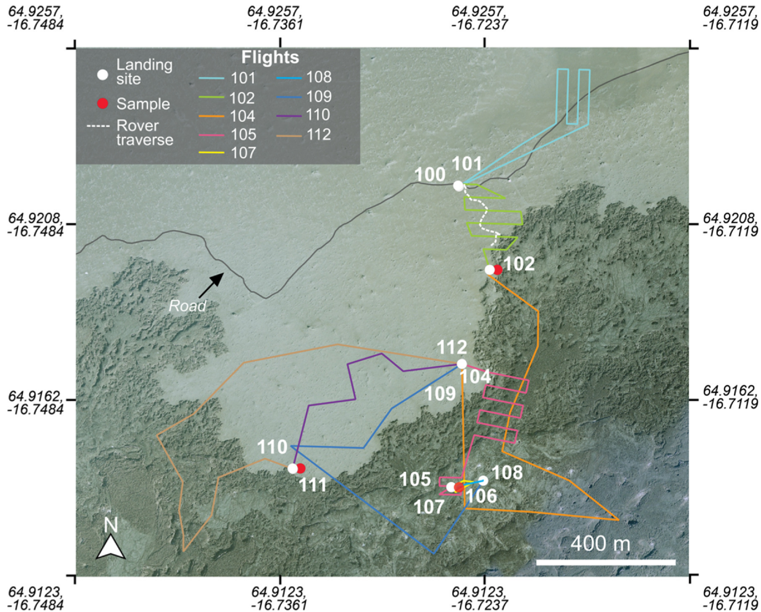
Figure 12. from Samantha Gwizd et al 2024 Planet. Sci. J. 5 doi:10.3847/PSJ/ad55f4 https://dx.doi.org/10.3847/PSJ/ad55f4 © 2024. The Author(s). Published by the American Astronomical Society.
