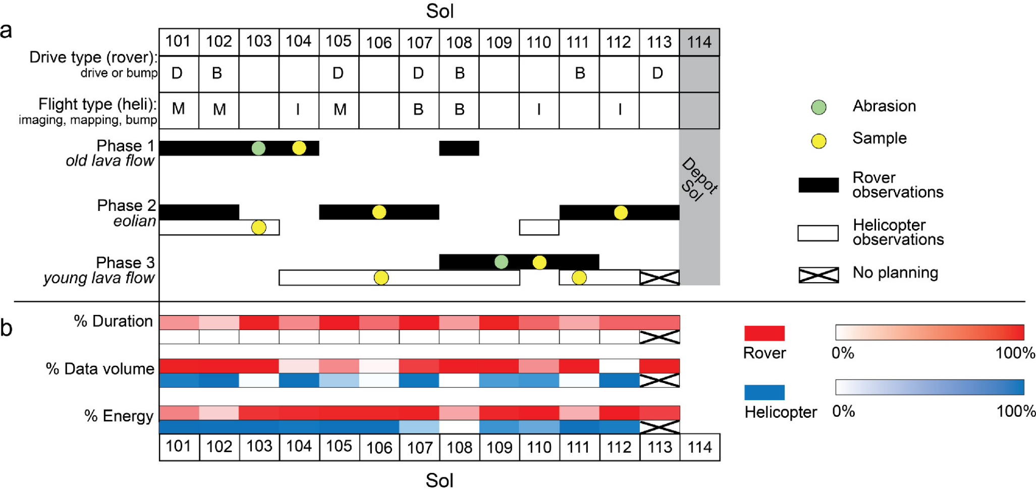
Figure 11. from Samantha Gwizd et al 2024 Planet. Sci. J. 5 doi:10.3847/PSJ/ad55f4 https://dx.doi.org/10.3847/PSJ/ad55f4 © 2024. The Author(s). Published by the American Astronomical Society.
