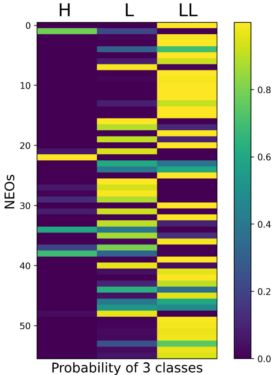
Figure 9. from Juan A. Sanchez et al 2024 Planet. Sci. J. 5 doi:10.3847/PSJ/ad445f https://dx.doi.org/10.3847/PSJ/ad445f © 2024. The Author(s). Published by the American Astronomical Society.
