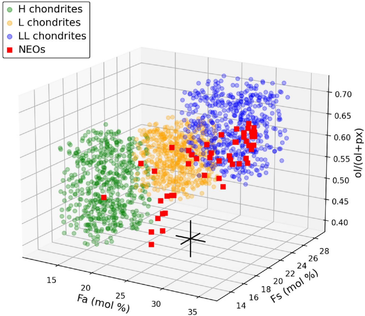
Figure 6. from Juan A. Sanchez et al 2024 Planet. Sci. J. 5 doi:10.3847/PSJ/ad445f https://dx.doi.org/10.3847/PSJ/ad445f © 2024. The Author(s). Published by the American Astronomical Society.
