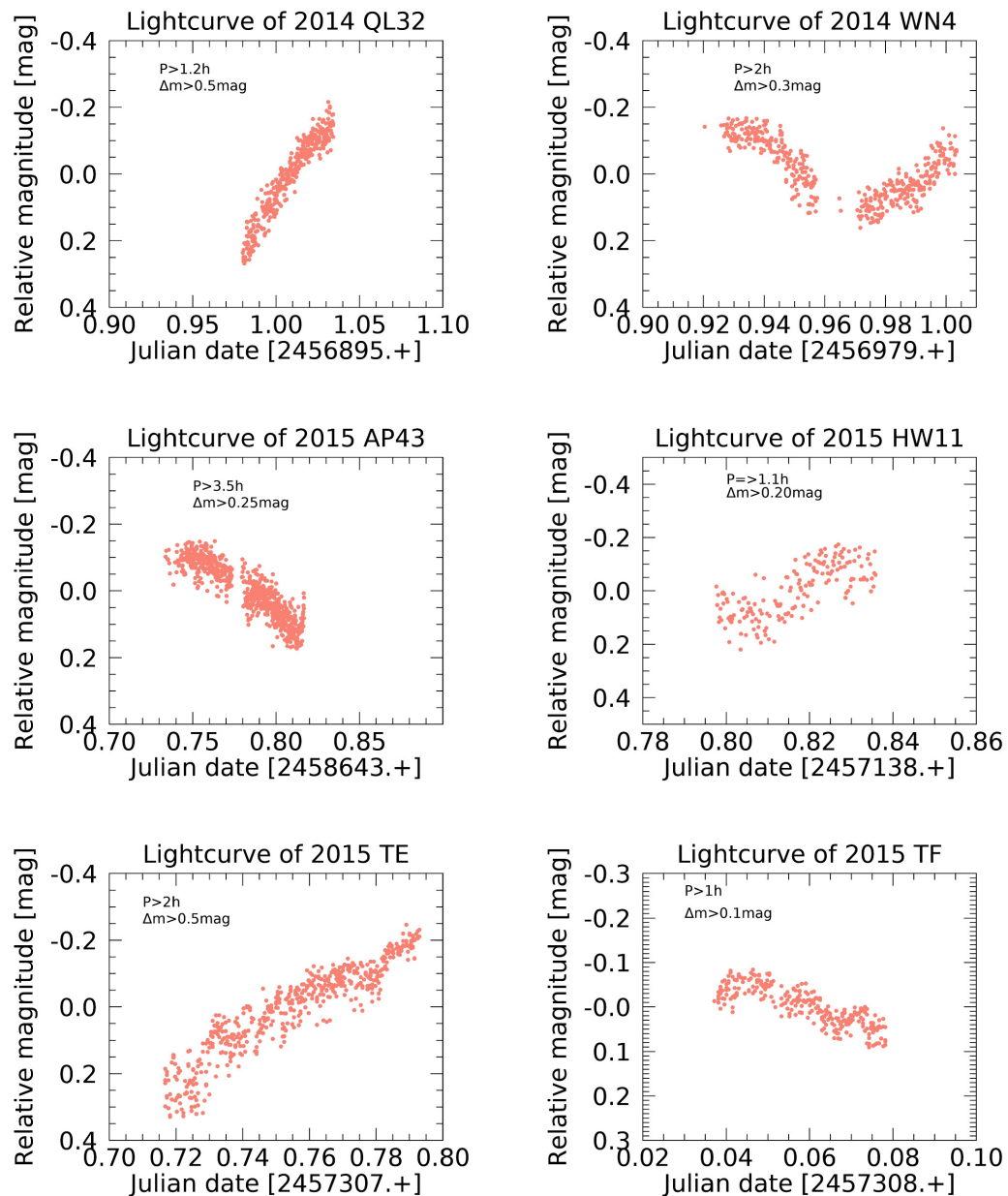
Figure 35. from Juan A. Sanchez et al 2024 Planet. Sci. J. 5 doi:10.3847/PSJ/ad445f https://dx.doi.org/10.3847/PSJ/ad445f © 2024. The Author(s). Published by the American Astronomical Society.
