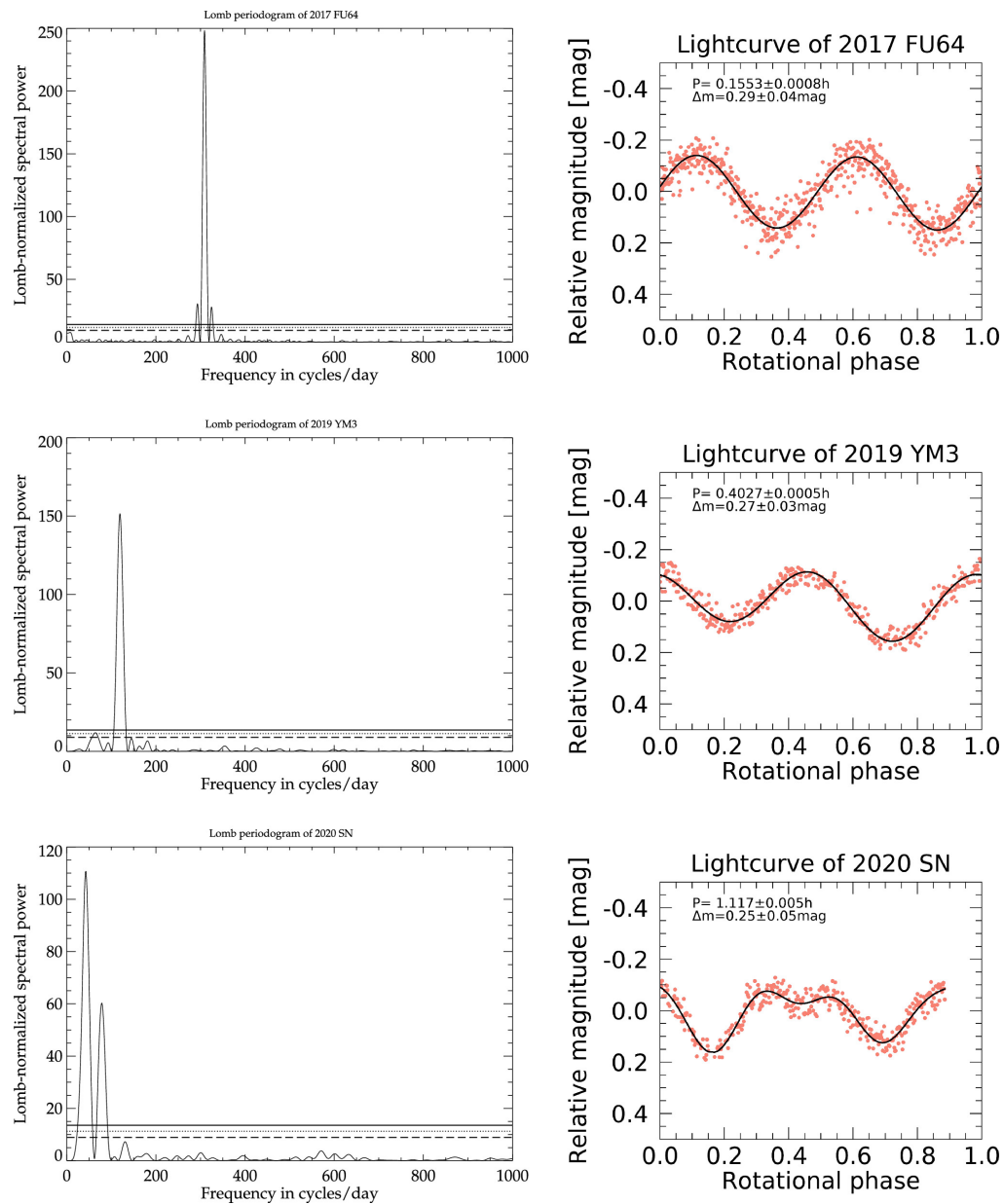
Figure 33. from Juan A. Sanchez et al 2024 Planet. Sci. J. 5 doi:10.3847/PSJ/ad445f https://dx.doi.org/10.3847/PSJ/ad445f © 2024. The Author(s). Published by the American Astronomical Society.
