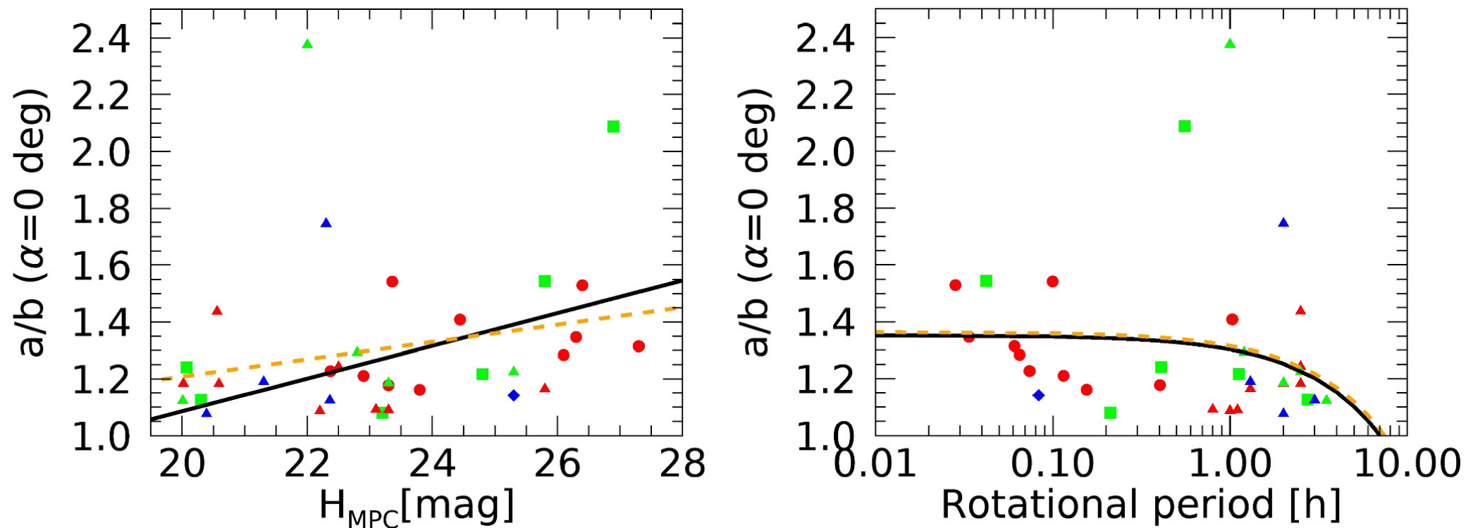
Figure 21. from Juan A. Sanchez et al 2024 Planet. Sci. J. 5 doi:10.3847/PSJ/ad445f https://dx.doi.org/10.3847/PSJ/ad445f © 2024. The Author(s). Published by the American Astronomical Society.
