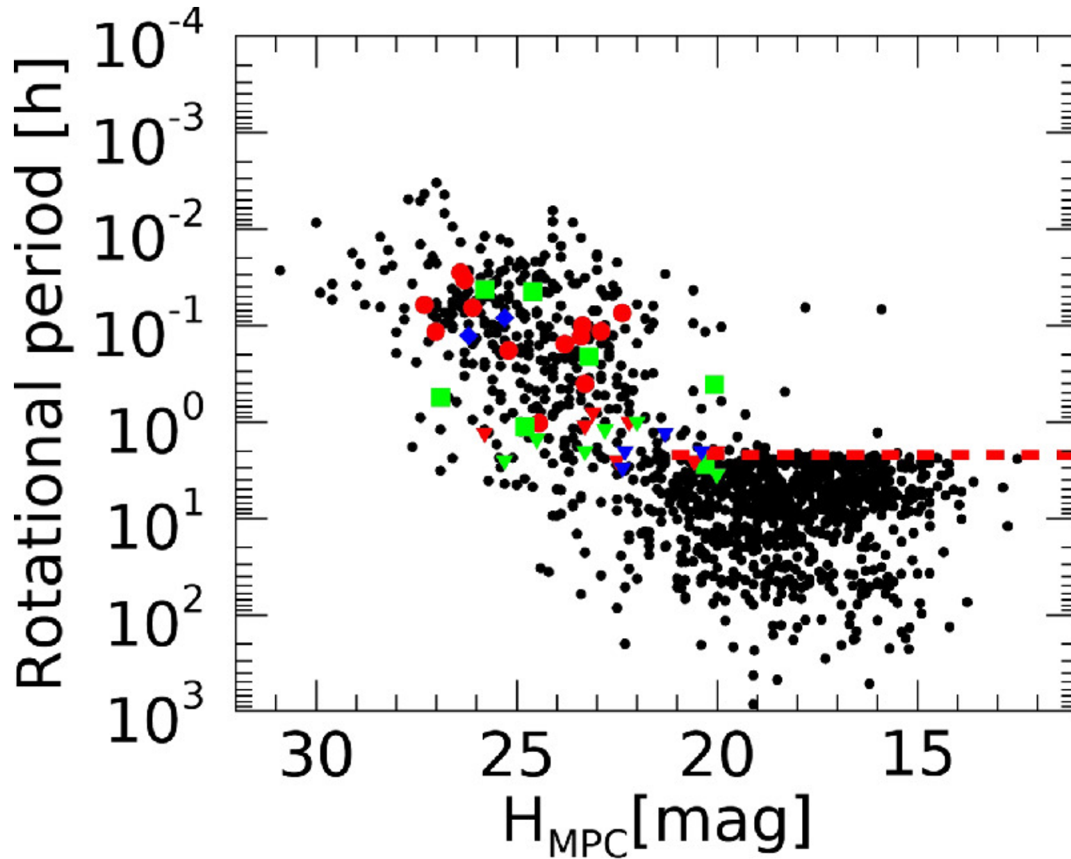
Figure 20. from Juan A. Sanchez et al 2024 Planet. Sci. J. 5 doi:10.3847/PSJ/ad445f https://dx.doi.org/10.3847/PSJ/ad445f © 2024. The Author(s). Published by the American Astronomical Society.
