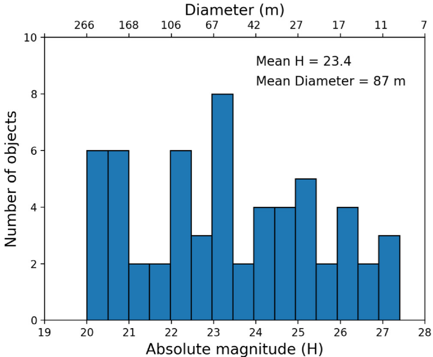
Figure 19. from Juan A. Sanchez et al 2024 Planet. Sci. J. 5 doi:10.3847/PSJ/ad445f https://dx.doi.org/10.3847/PSJ/ad445f © 2024. The Author(s). Published by the American Astronomical Society.
