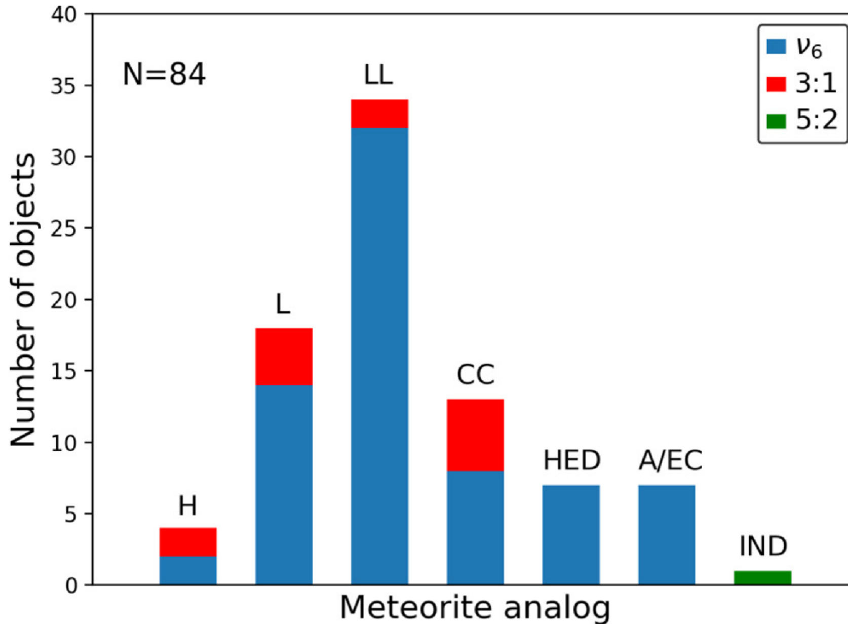
Figure 18. from Juan A. Sanchez et al 2024 Planet. Sci. J. 5 doi:10.3847/PSJ/ad445f https://dx.doi.org/10.3847/PSJ/ad445f © 2024. The Author(s). Published by the American Astronomical Society.
