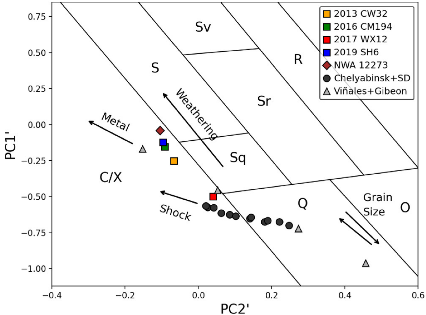
Figure 16. from Juan A. Sanchez et al 2024 Planet. Sci. J. 5 doi:10.3847/PSJ/ad445f https://dx.doi.org/10.3847/PSJ/ad445f © 2024. The Author(s). Published by the American Astronomical Society.
