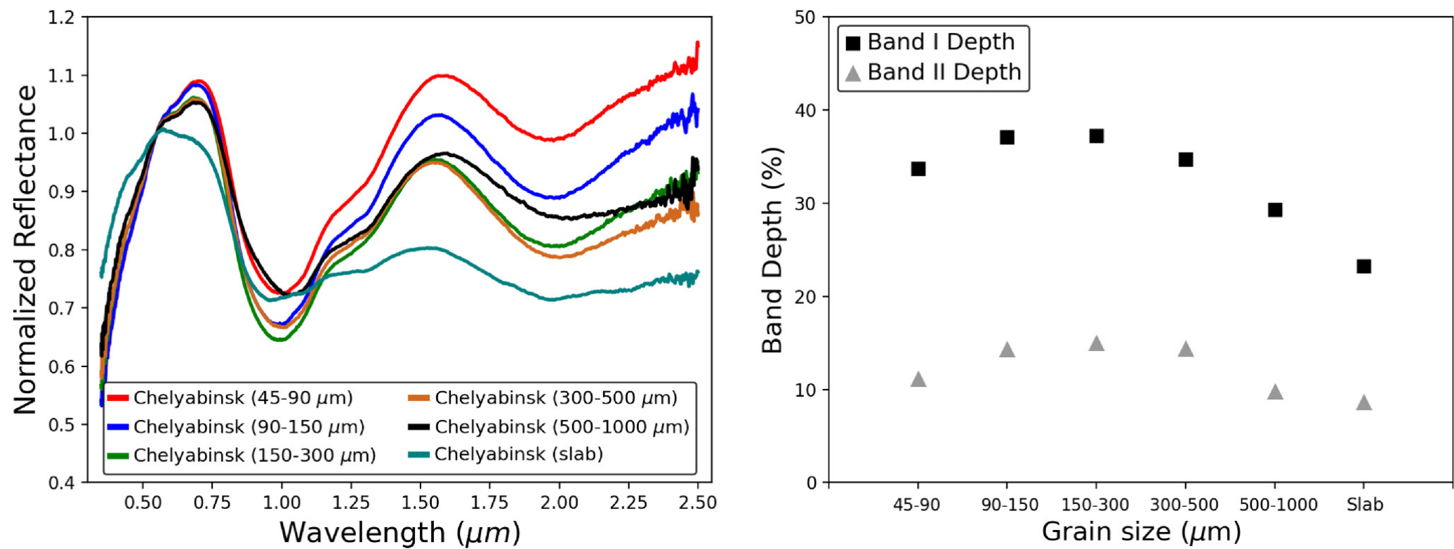
Figure 14. from Juan A. Sanchez et al 2024 Planet. Sci. J. 5 doi:10.3847/PSJ/ad445f https://dx.doi.org/10.3847/PSJ/ad445f © 2024. The Author(s). Published by the American Astronomical Society.
