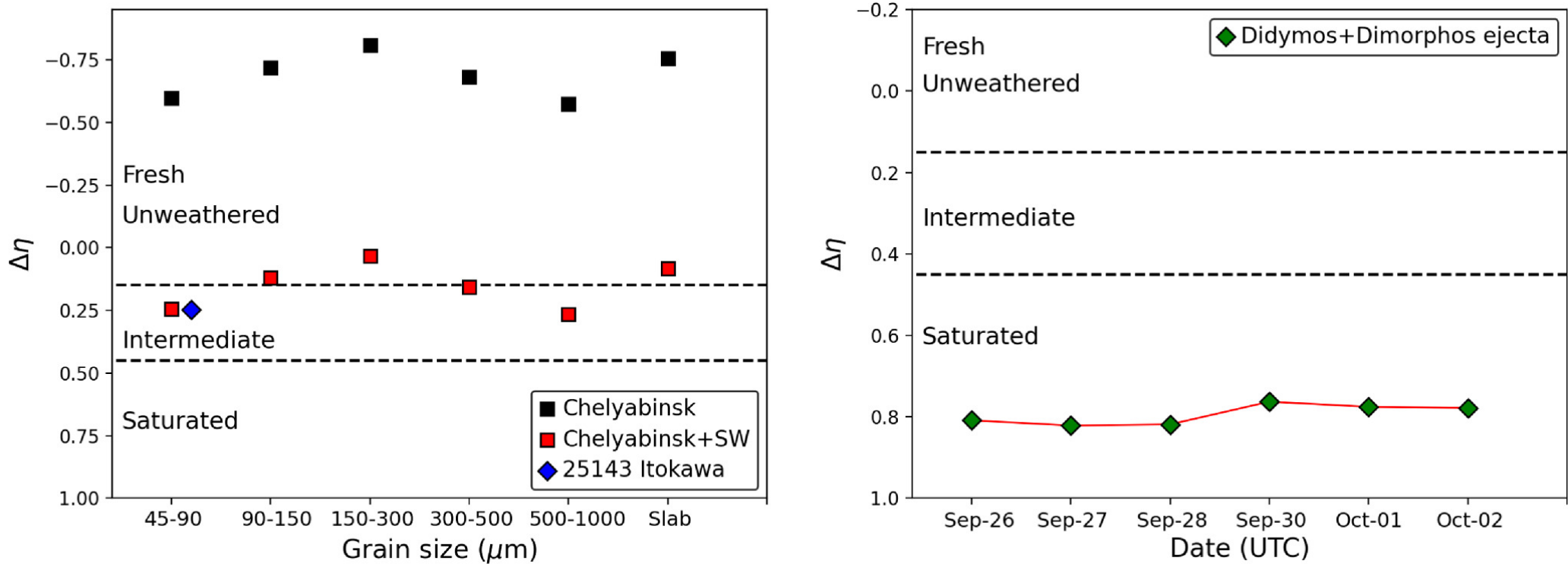
Figure 13. from Juan A. Sanchez et al 2024 Planet. Sci. J. 5 doi:10.3847/PSJ/ad445f https://dx.doi.org/10.3847/PSJ/ad445f © 2024. The Author(s). Published by the American Astronomical Society.
