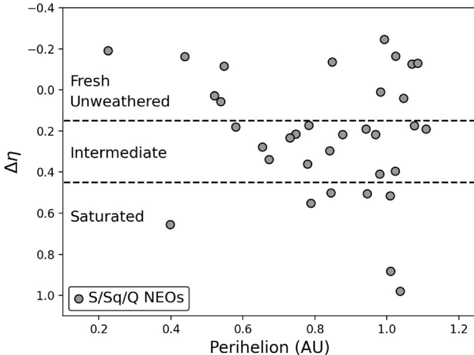
Figure 12. from Juan A. Sanchez et al 2024 Planet. Sci. J. 5 doi:10.3847/PSJ/ad445f https://dx.doi.org/10.3847/PSJ/ad445f © 2024. The Author(s). Published by the American Astronomical Society.
