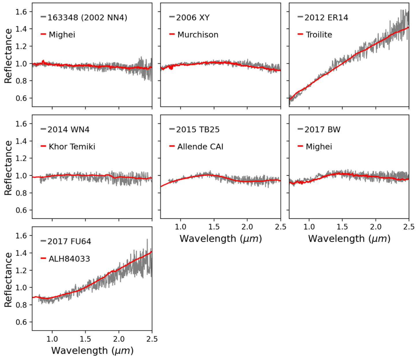
Figure 11. from Juan A. Sanchez et al 2024 Planet. Sci. J. 5 doi:10.3847/PSJ/ad445f https://dx.doi.org/10.3847/PSJ/ad445f © 2024. The Author(s). Published by the American Astronomical Society.
