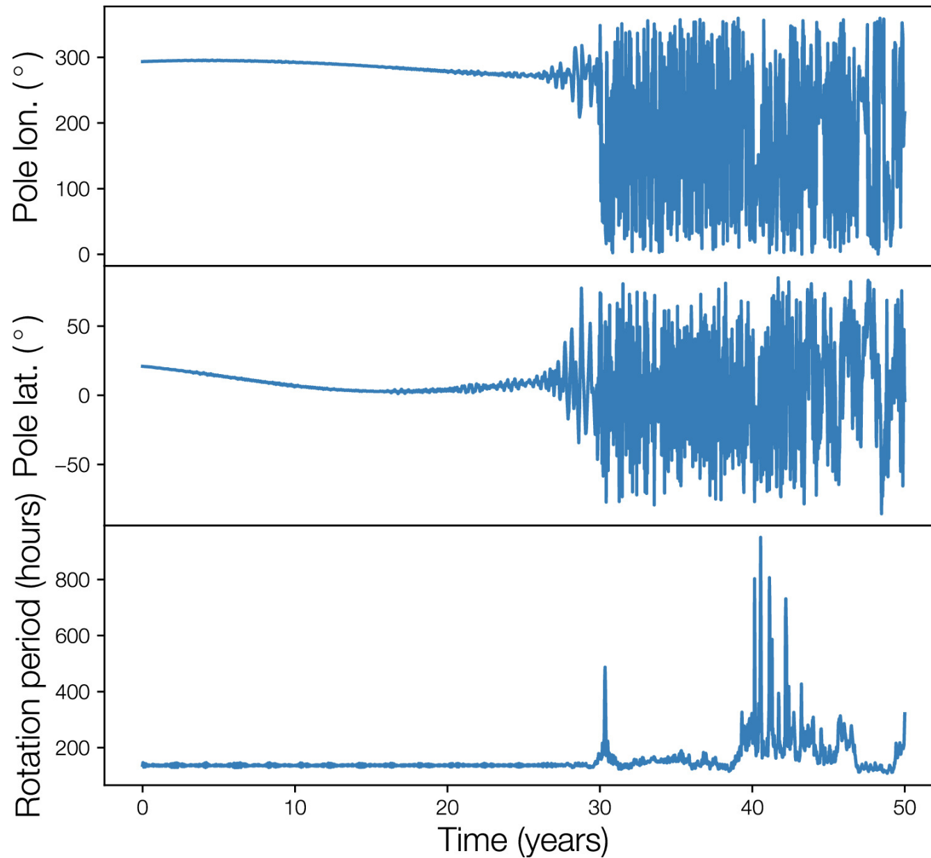
Figure 8. from Benjamin C. N. Proudfoot et al 2024 Planet. Sci. J. 5 doi:10.3847/PSJ/ad26e9 https://dx.doi.org/10.3847/PSJ/ad26e9 © 2024. The Author(s). Published by the American Astronomical Society.
