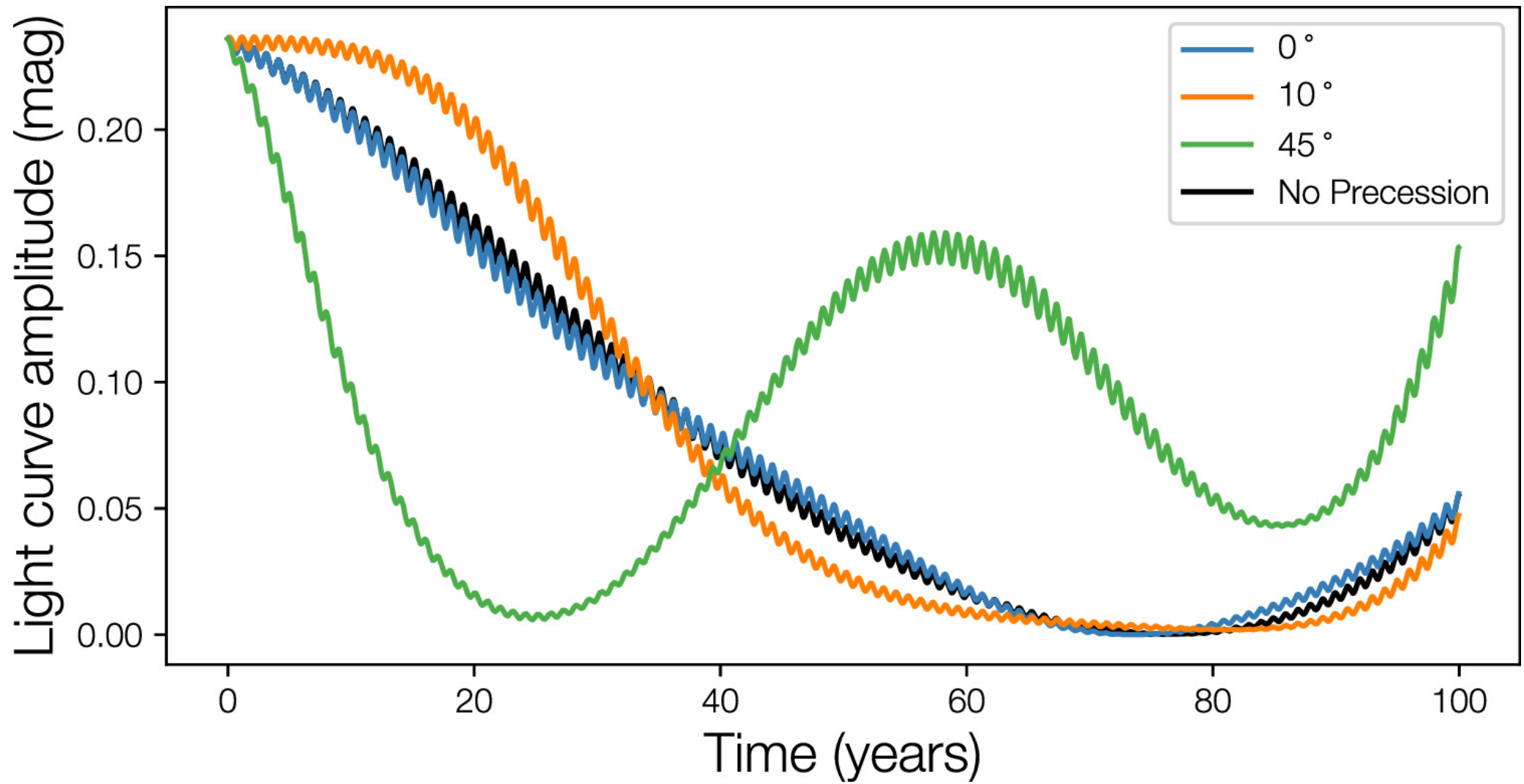
Figure 7. from Benjamin C. N. Proudfoot et al 2024 Planet. Sci. J. 5 doi:10.3847/PSJ/ad26e9 https://dx.doi.org/10.3847/PSJ/ad26e9 © 2024. The Author(s). Published by the American Astronomical Society.
