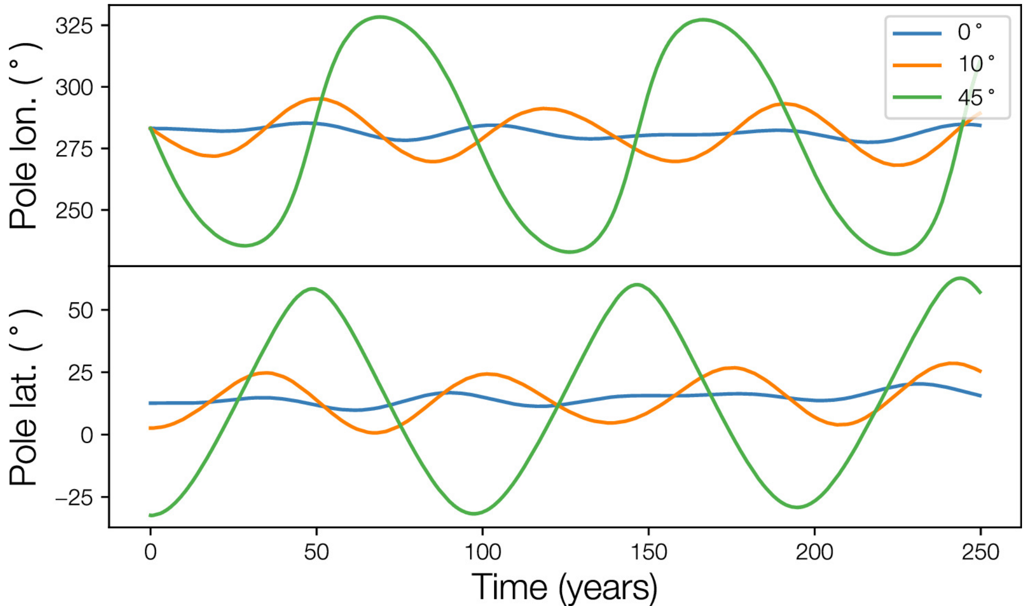
Figure 6. from Benjamin C. N. Proudfoot et al 2024 Planet. Sci. J. 5 doi:10.3847/PSJ/ad26e9 https://dx.doi.org/10.3847/PSJ/ad26e9 © 2024. The Author(s). Published by the American Astronomical Society.
