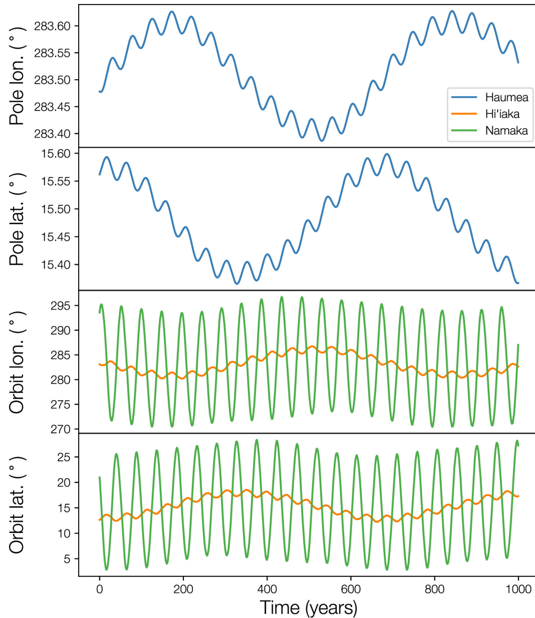
Figure 5. from Benjamin C. N. Proudfoot et al 2024 Planet. Sci. J. 5 doi:10.3847/PSJ/ad26e9 https://dx.doi.org/10.3847/PSJ/ad26e9 © 2024. The Author(s). Published by the American Astronomical Society.
