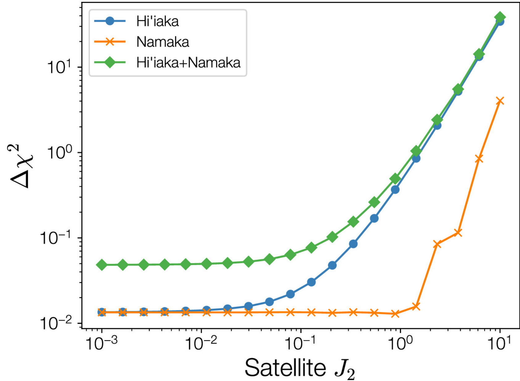
Figure 4. from Benjamin C. N. Proudfoot et al 2024 Planet. Sci. J. 5 doi:10.3847/PSJ/ad26e9 https://dx.doi.org/10.3847/PSJ/ad26e9 © 2024. The Author(s). Published by the American Astronomical Society.
