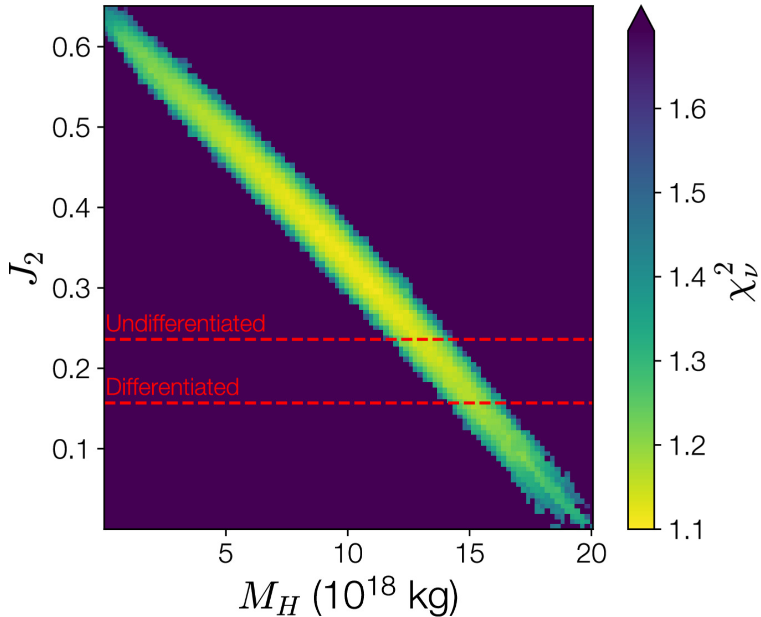
Figure 3. from Benjamin C. N. Proudfoot et al 2024 Planet. Sci. J. 5 doi:10.3847/PSJ/ad26e9 https://dx.doi.org/10.3847/PSJ/ad26e9 © 2024. The Author(s). Published by the American Astronomical Society.
