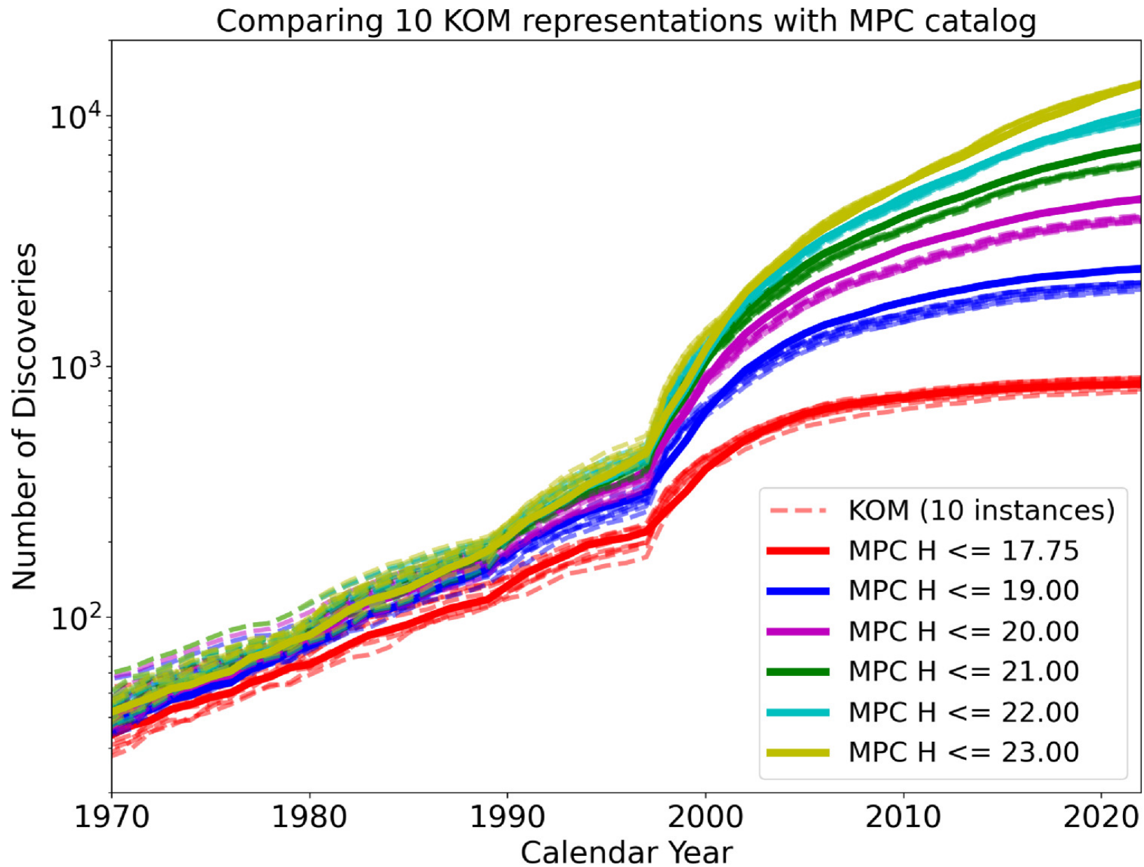
Figure 8. from Tommy Grav et al 2023 Planet. Sci. J. 4 doi:10.3847/PSJ/ad072e https://dx.doi.org/10.3847/PSJ/ad072e © 2023. The Author(s). Published by the American Astronomical Society.
