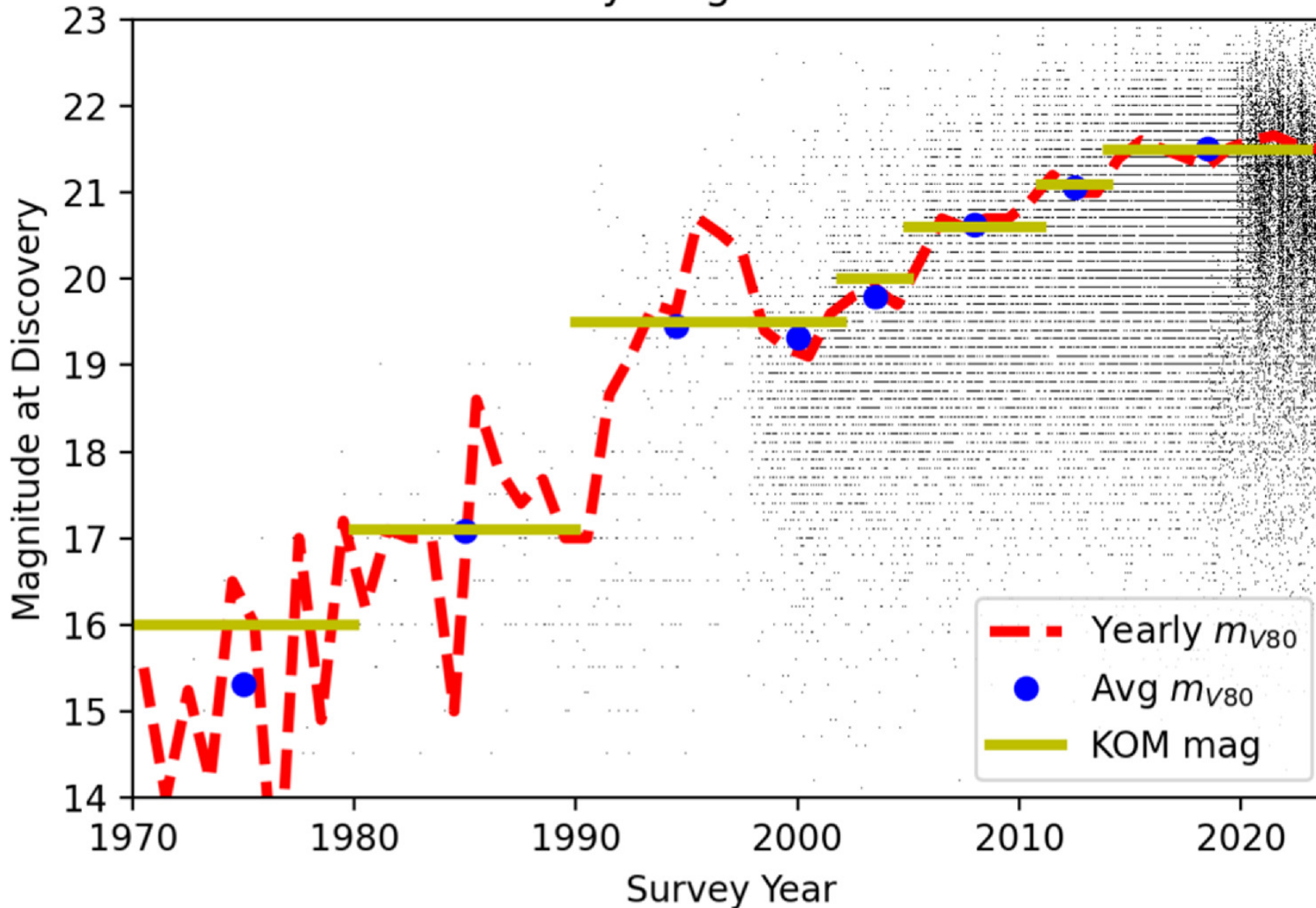
Figure 7. from Tommy Grav et al 2023 Planet. Sci. J. 4 doi:10.3847/PSJ/ad072e https://dx.doi.org/10.3847/PSJ/ad072e © 2023. The Author(s). Published by the American Astronomical Society.
